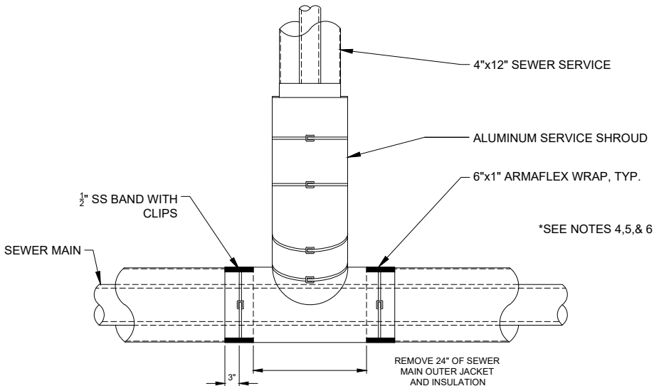
5 SEWER SERVICE CONNECTION AT MAIN PLAN VIEW M-201 SCALE: NTS
