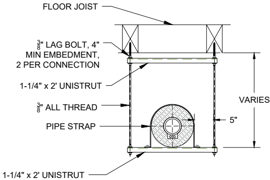
2 SERVICE PIPE HANGER M-201 SCALE: NTS
