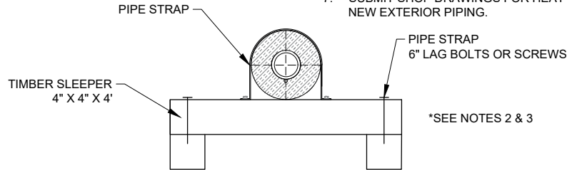
3 SERVICE PIPE GROUND SUPPORT M-201 SCALE: NTS
