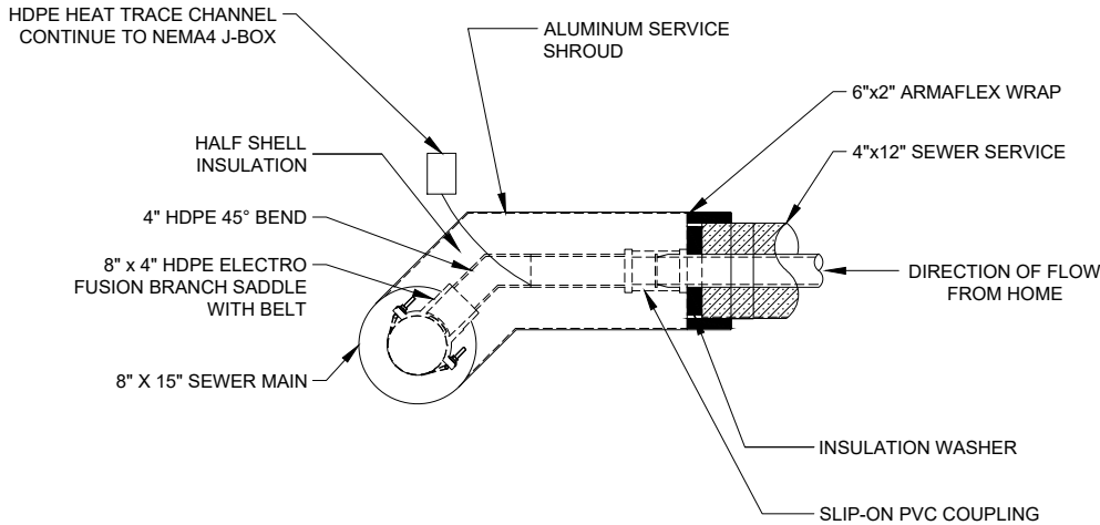
4 SEWER SERVICE CONNECTION AT MAIN SECTION VIEW M-201 SCALE: NTS
