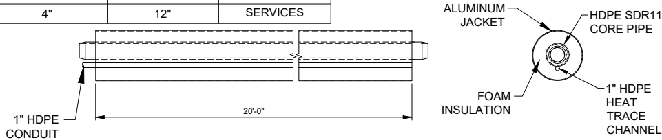
1 ARCTIC SEWER SERVICE PIPE M-201 SCALE: NTS
