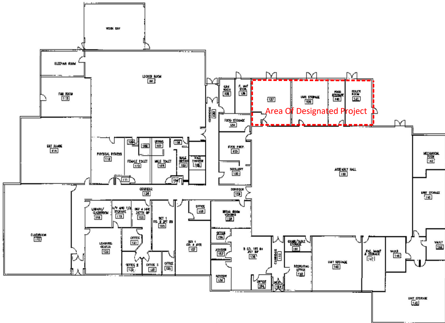
BUILDING FLOOR PLAN SCALE: 1" = 10'-0"
