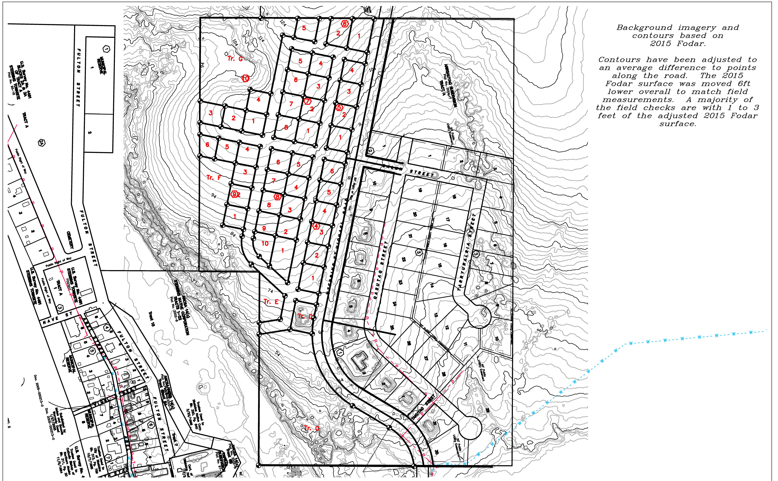
SHEET 1 - OVERVIEW (1"=250')
