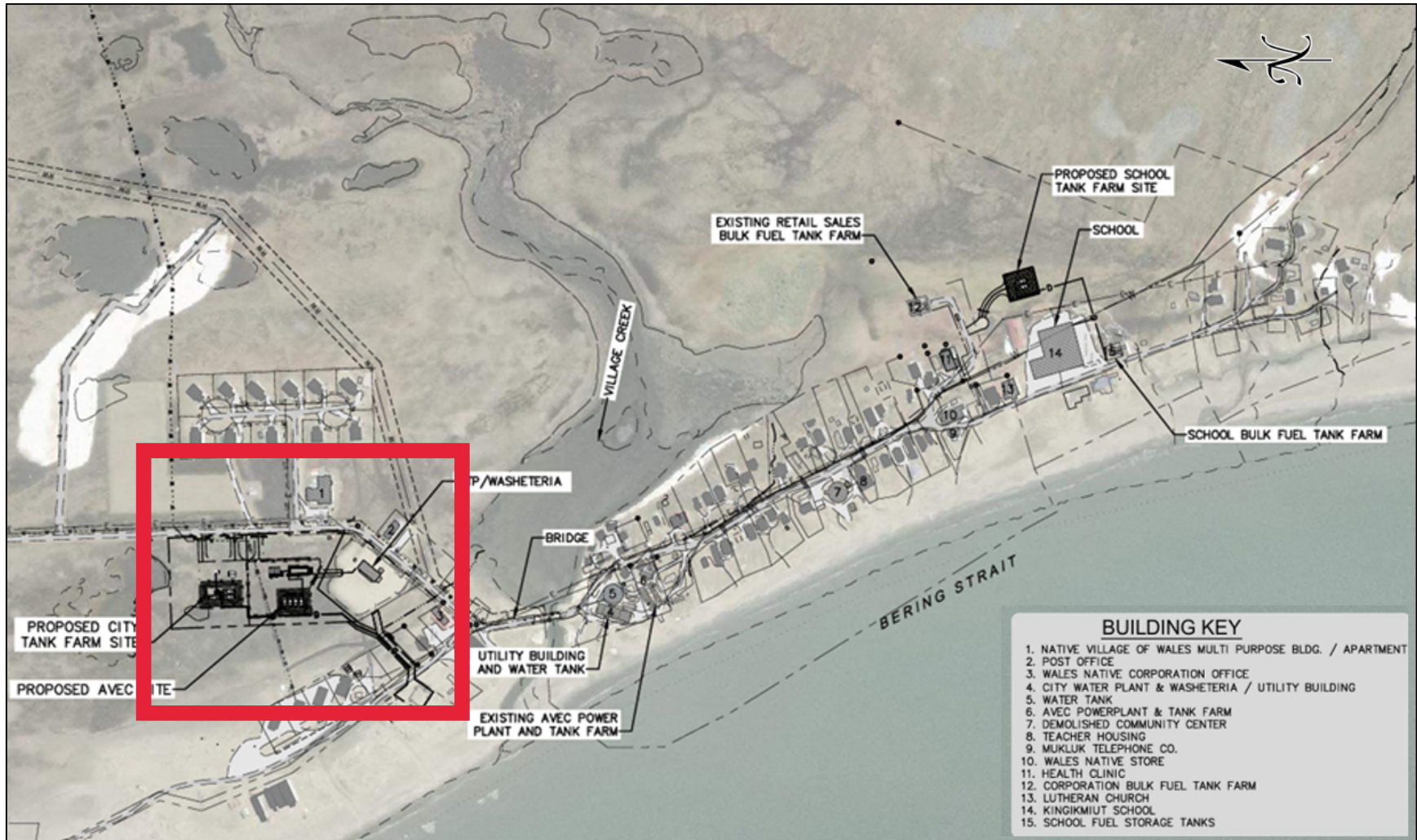
Figure 2. Wales Community Map Showing Existing and Proposed Tank Farm Locations and Other Infrastructure
