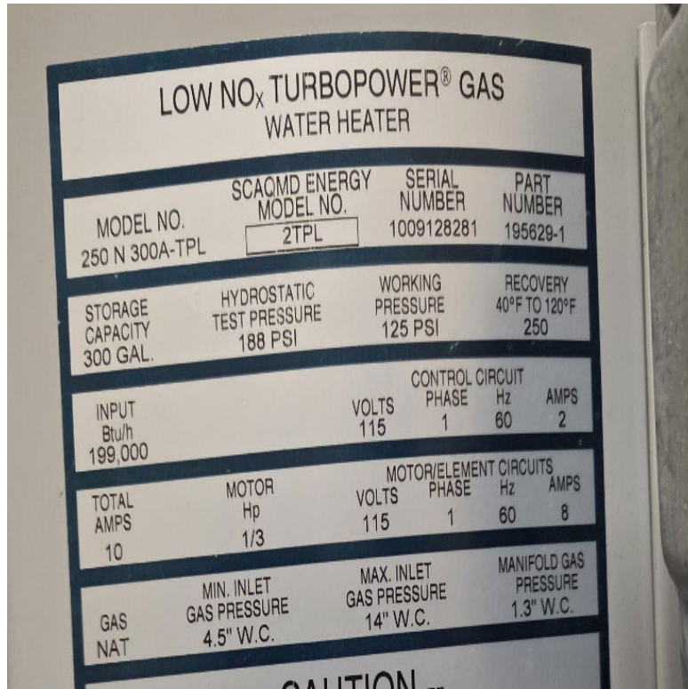
Figure 1. Existing Water Heater Data Plate
