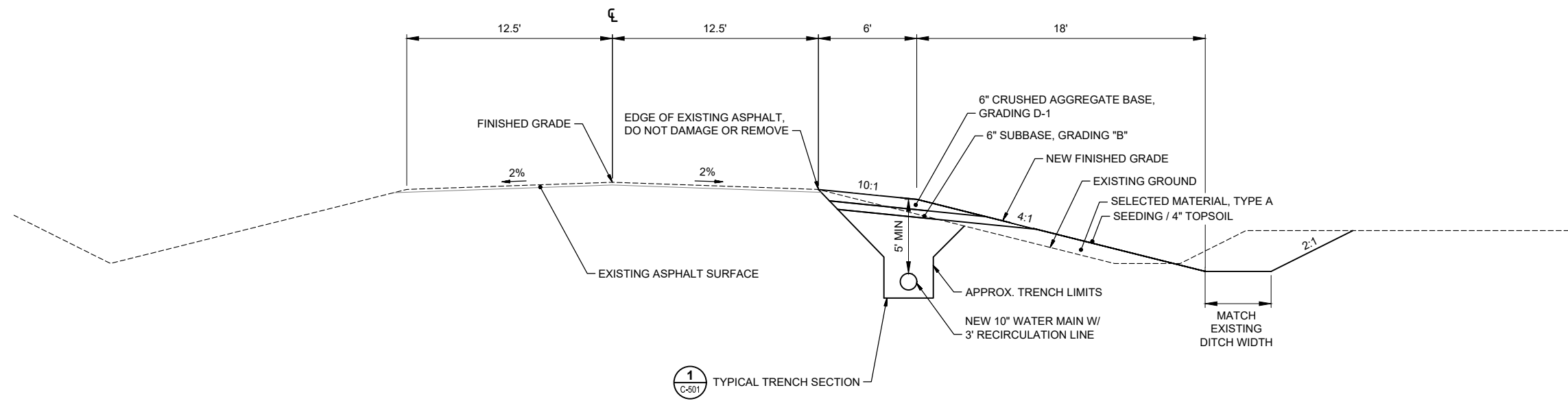
1 AIRPORT ROAD TYPICAL SECTION C-401 SCALE: N.T.S
