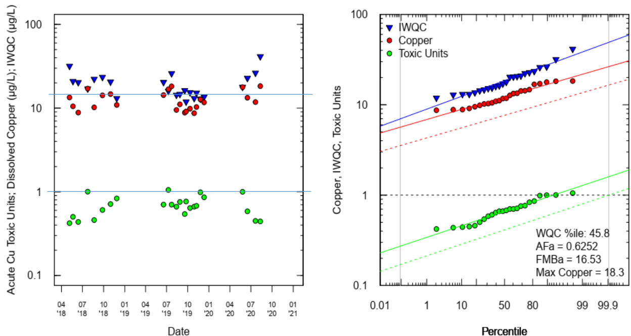
Figure 3. An example dataset for FMB calculations showing acute IWQC, Cu concentrations, and toxic units as either a time-series (left) or probability plot (right).
