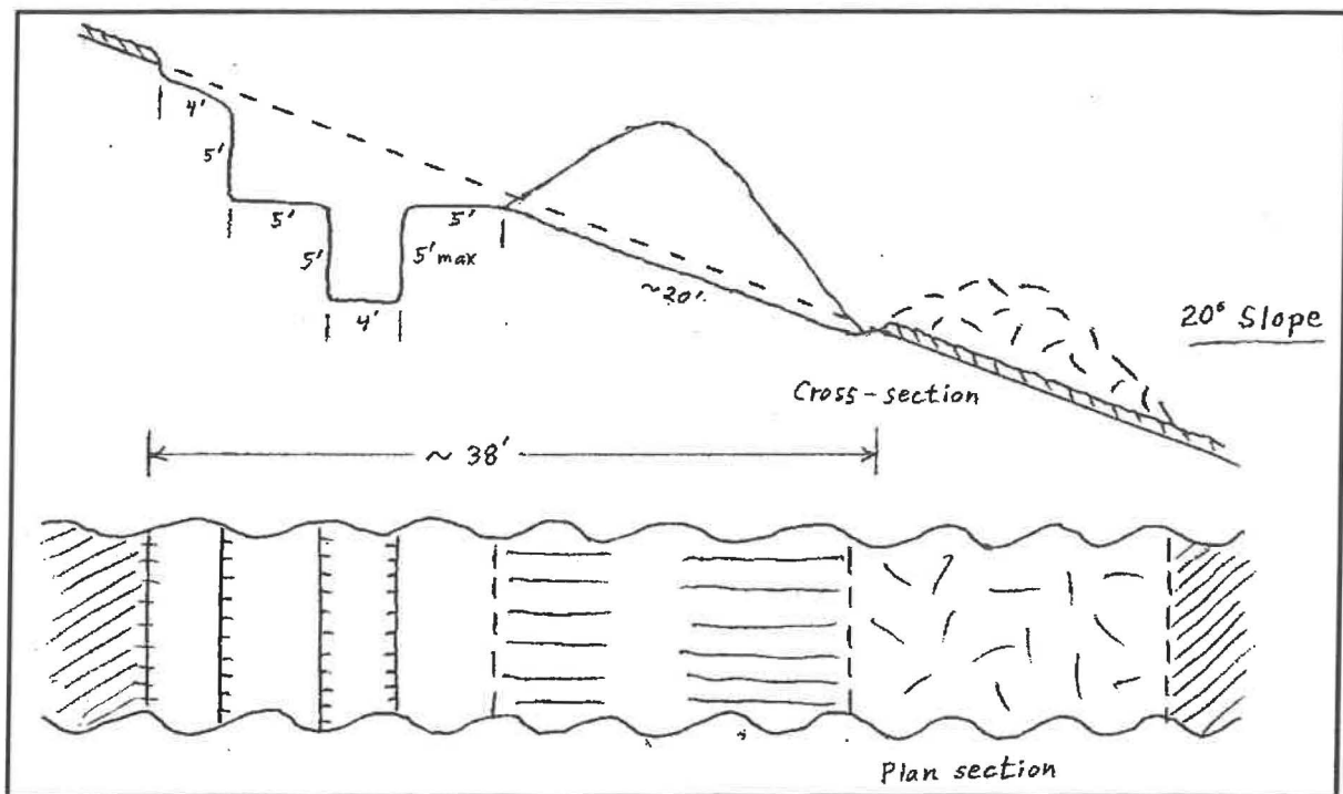
Figure 4. Cross-section through double-bench trench on 20° slope
