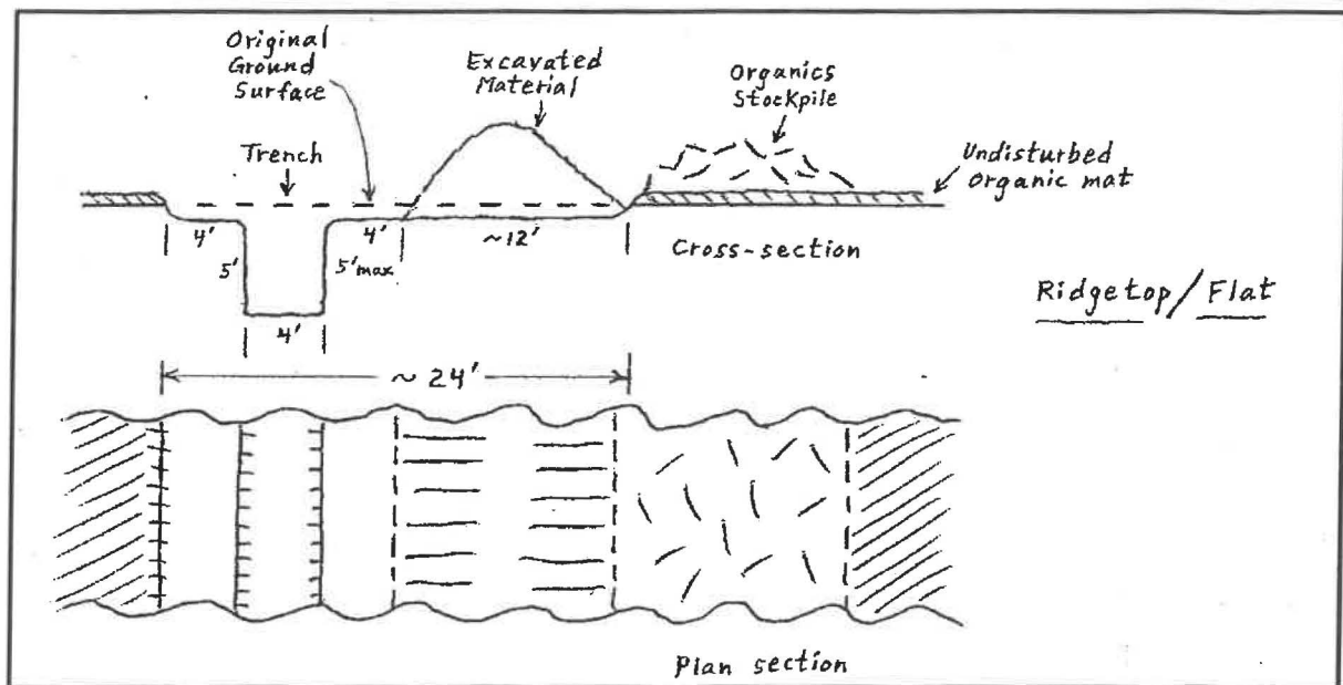
Figure 3. Cross-section through single-bench trench on gentle slope
