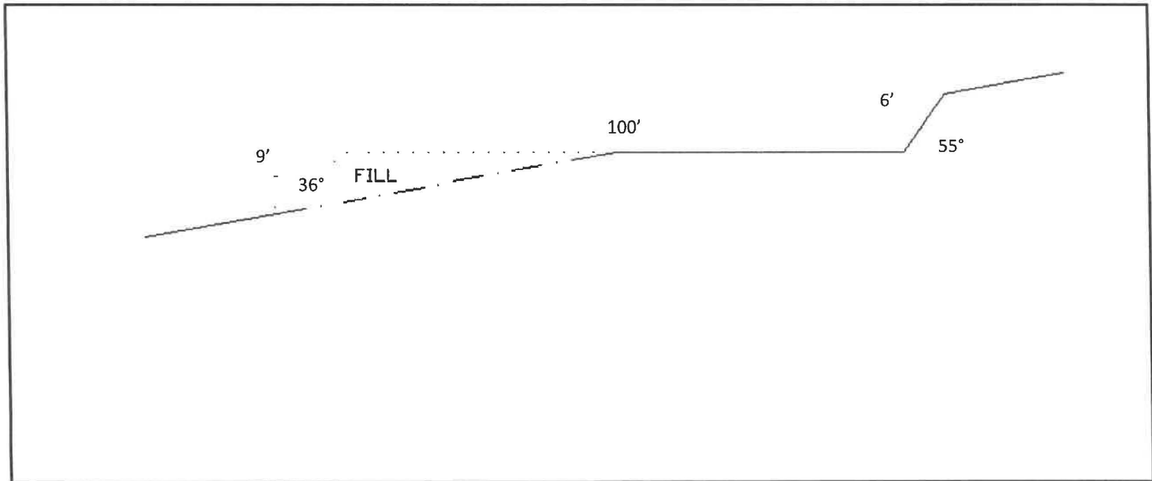
Figure 2. Cross-section through typical drill pad
