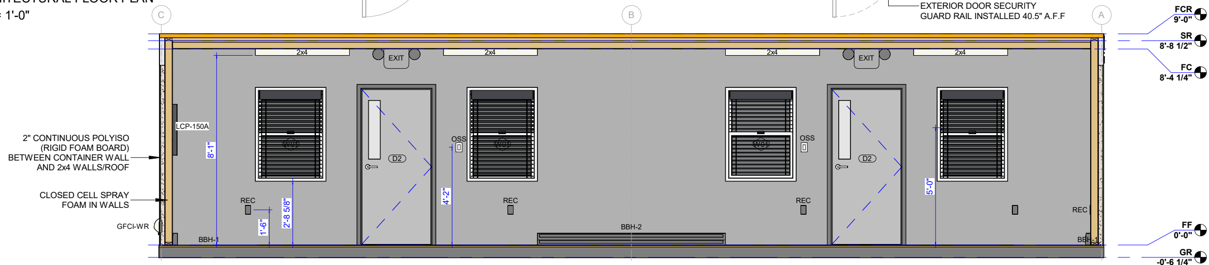
2 REAR SECTION VIEW 1/4" = 1'-0"
