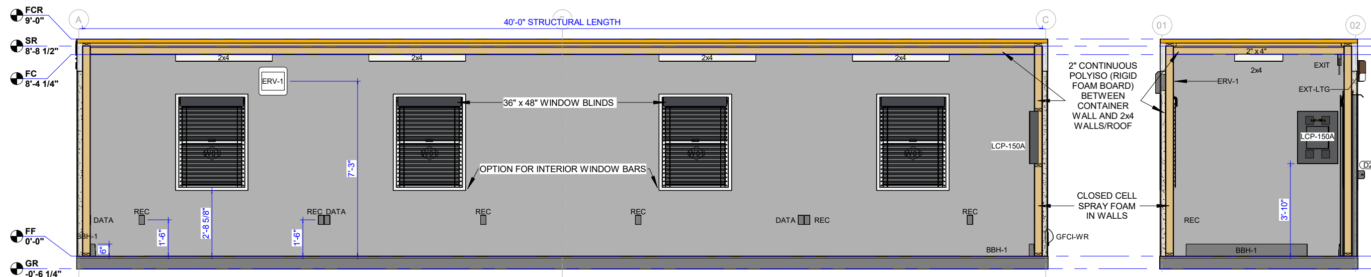
3 FRONT SECTION VIEW 1/4" = 1'-0"
