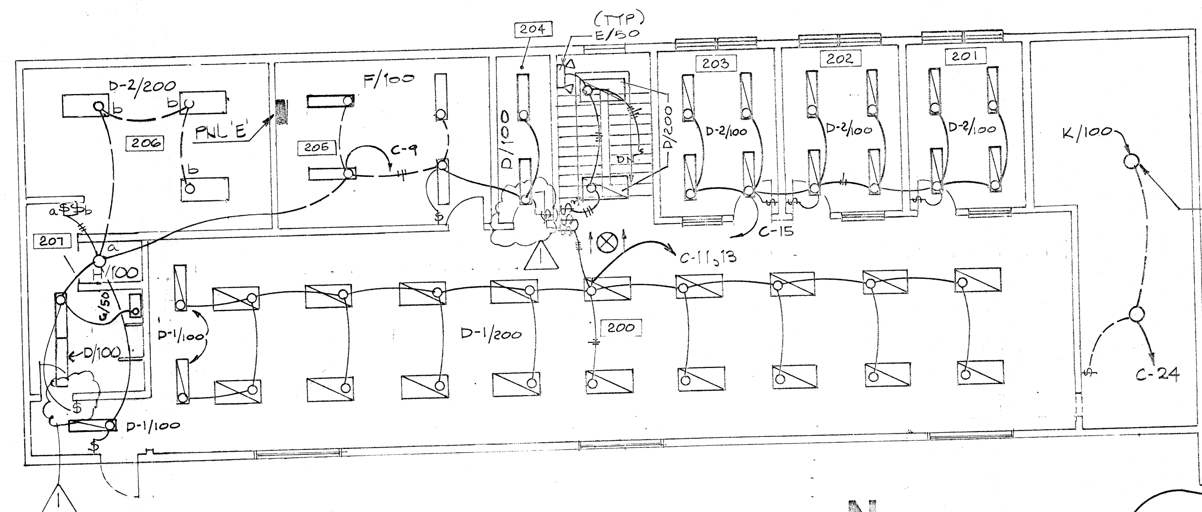
2 SECOND FLOOR LIGHTING PLAN
