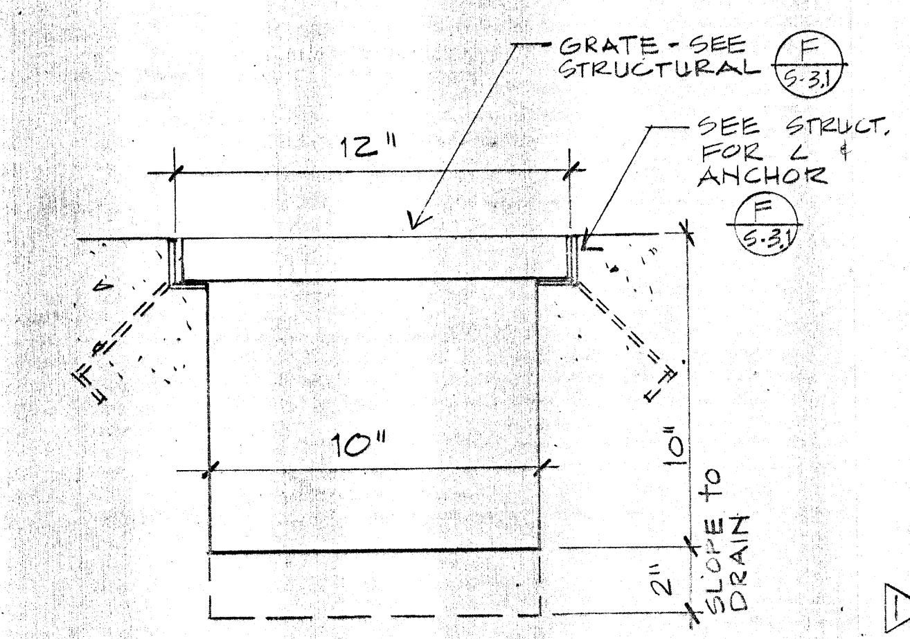
1 TRENCH DETAIL SEE ALSO STRUCT. DETAIL F/5.3.1
