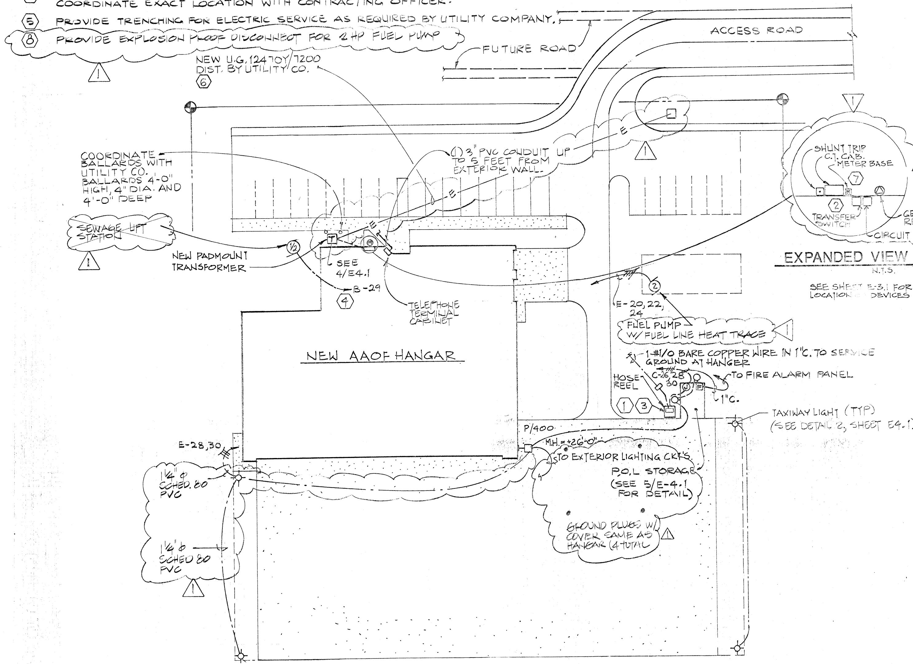
ELECTRICAL SITE PLAN
