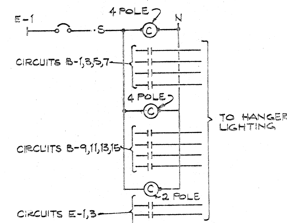
HANGER LIGHTING CONTROL DIAGRAM
