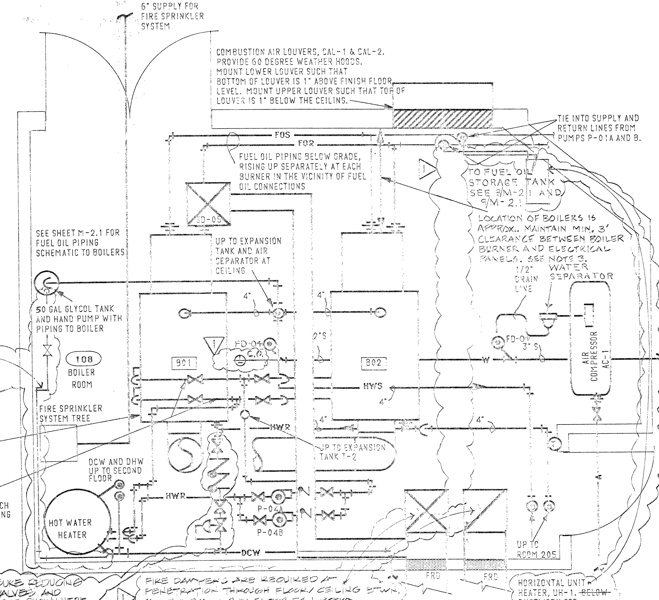
3 FIRST FLOOR MECHANICAL ROOM 1/2" = 1'-0"
