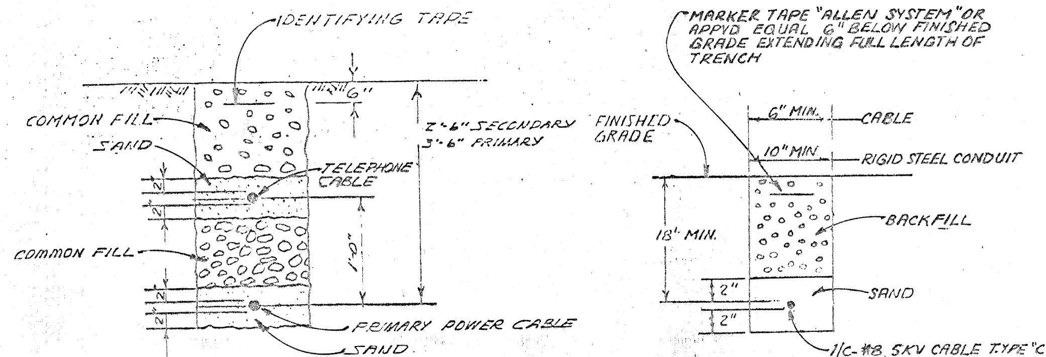
TRENCH DETAIL
