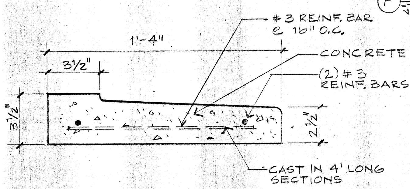
2 SPLASH BLOCK 3" = 1'-0"
