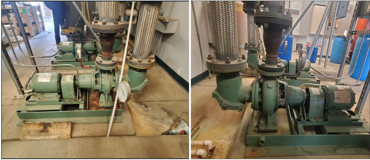
Figure 3 & 4. Profile View, Pump Motor, Elbow with Flange Connections
