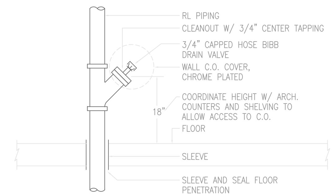
2 RAIN LEADER CLEANOUT DETAIL NO SCALE
