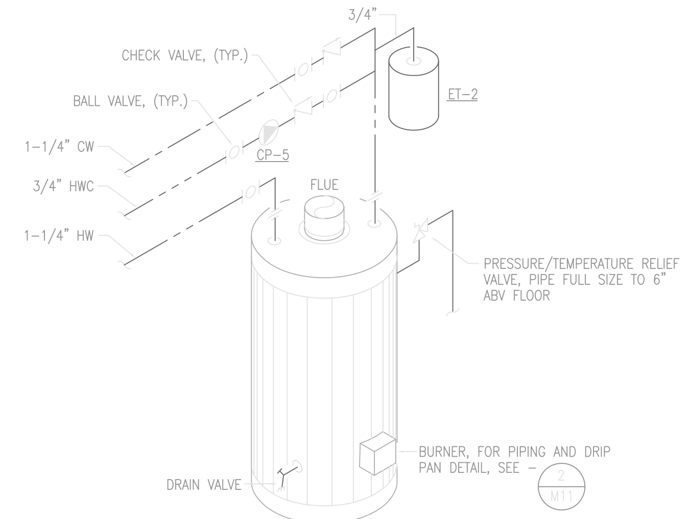
4 WATER HEATER PIPING DETAIL NO SCALE
