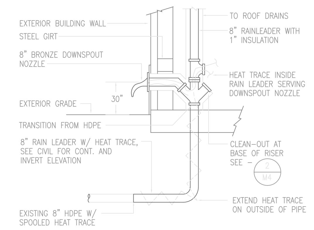
3 RAIN LEADER DETAIL NO SCALE
