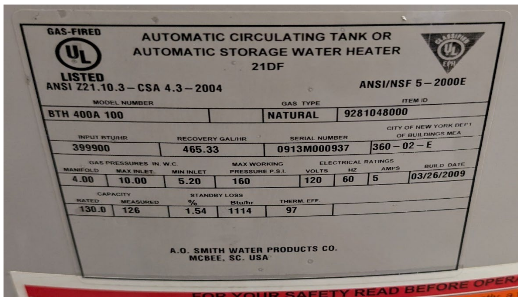
Figure 1: Data Plate for WH-1
