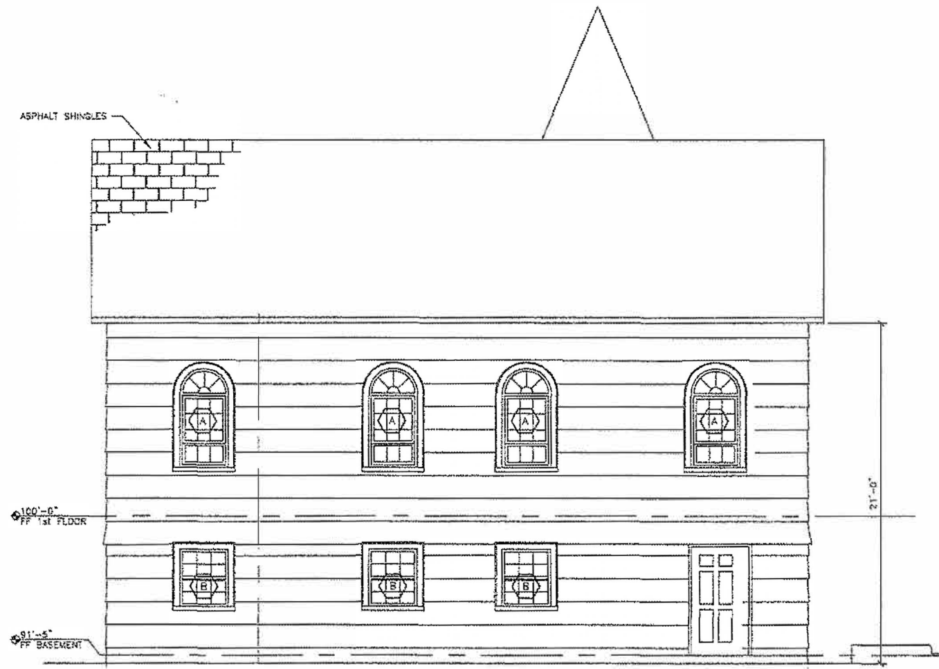
2 SOUTH EXTERIOR ELEVATION SCALE: 0 2' 4' 8'
