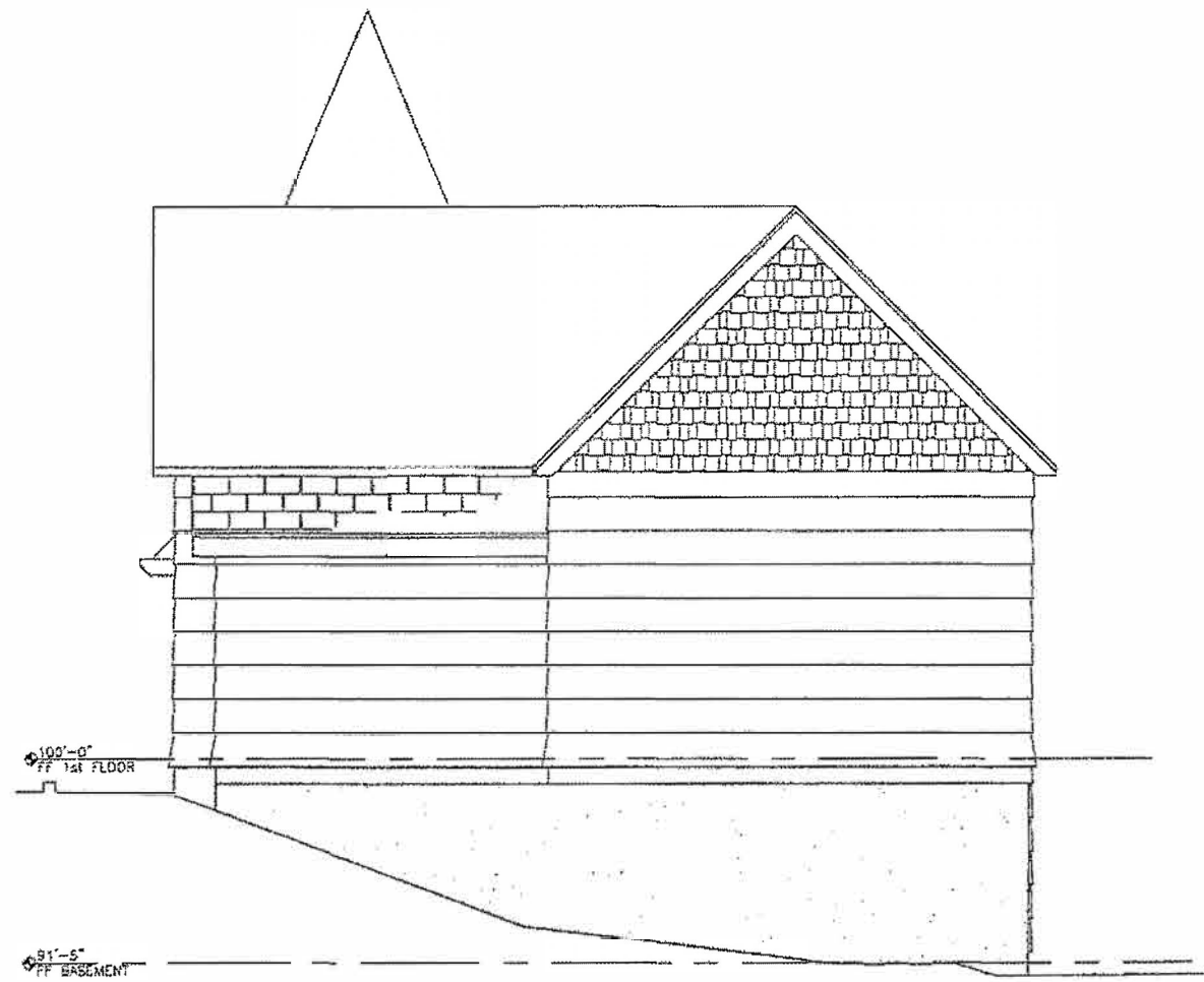
1 WEST EXTERIOR ELEVATION SCALE: 0 2' 4' 8'
