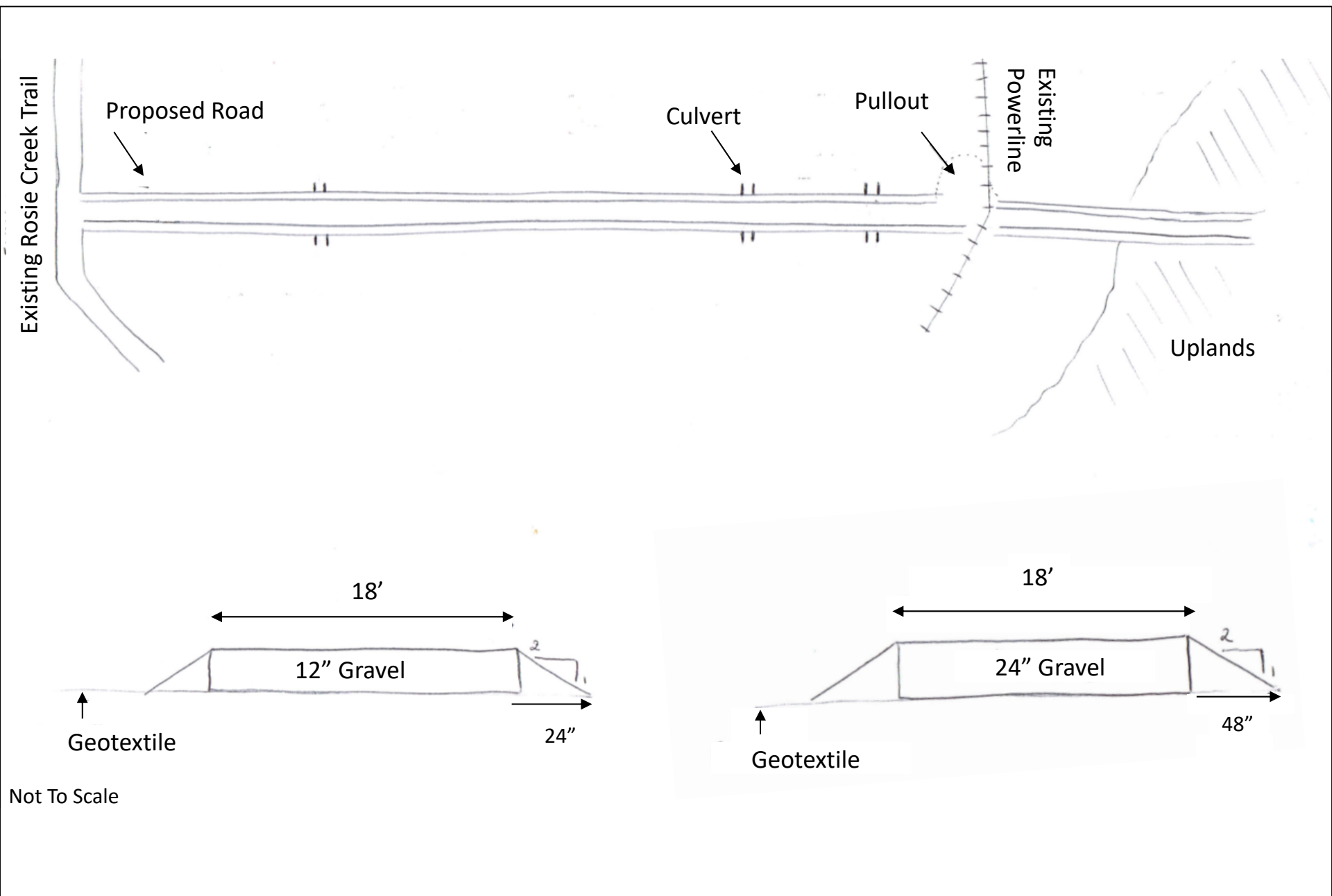
Sheet 3: Fairbanks Gravel Road and Gravel Harvest Project Road Plans
