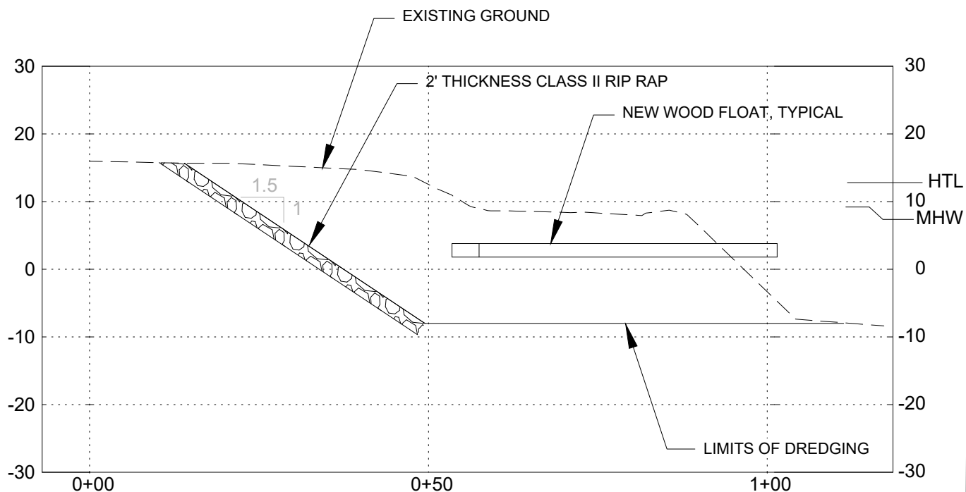
HORIZONTAL SCALE 1" = 20' SECTION VIEW A-A FLOAT AND DREDGING
