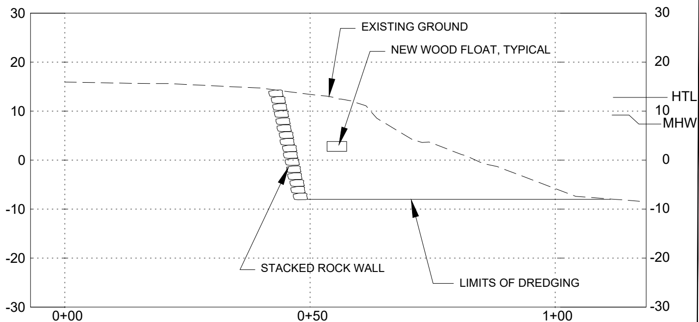
HORIZONTAL SCALE 1" = 20' SECTION VIEW B-B STACKED ROCK WALL AND DREDGING
