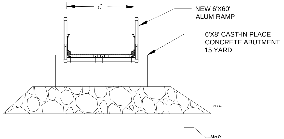
GANGWAY SECTION VIEW
