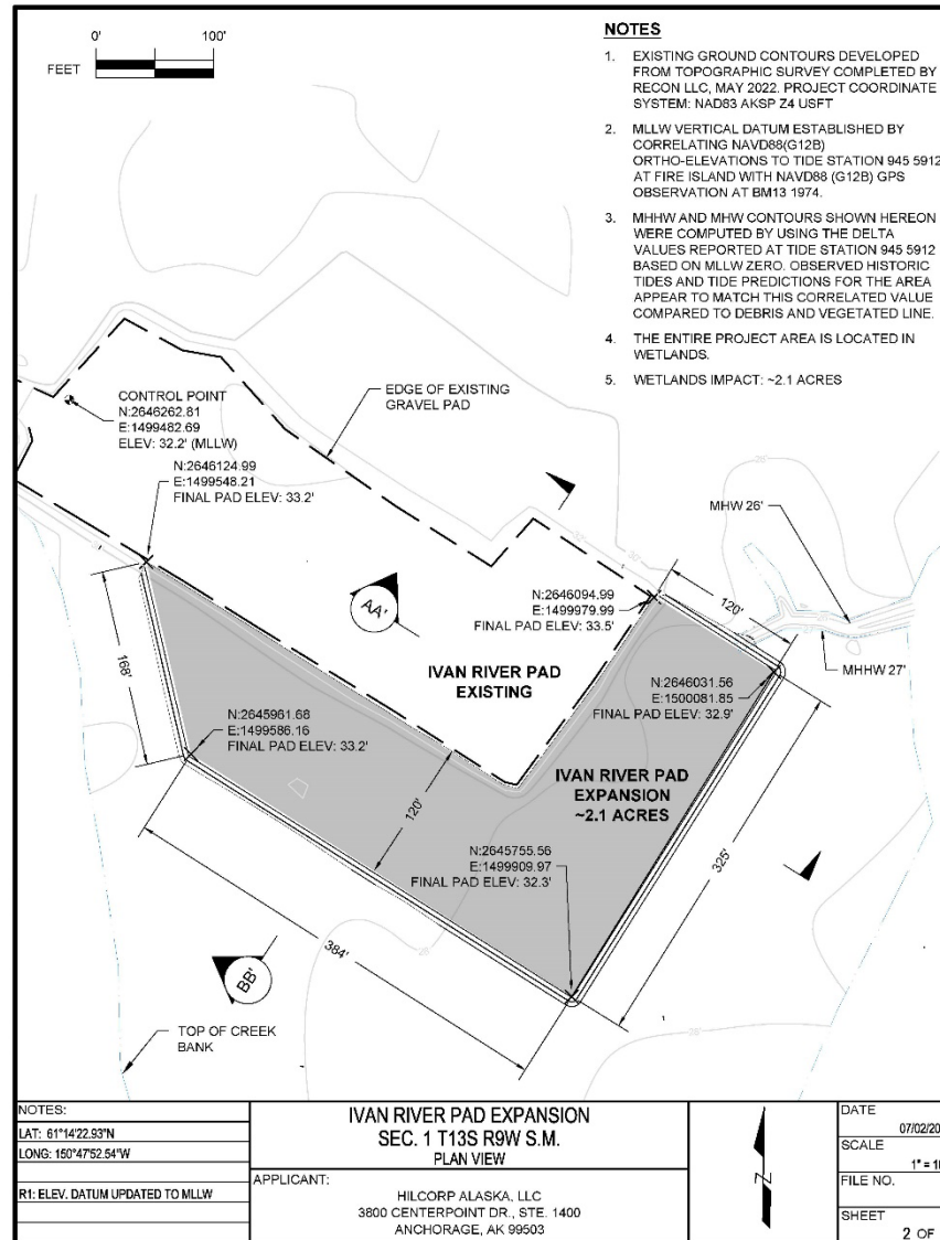
Figure 2: Ivan River Unit Pad Plan View
