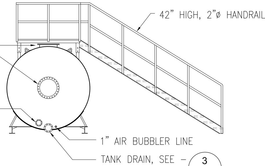
END VIEW (SKID SHOWN AS SECTION)
