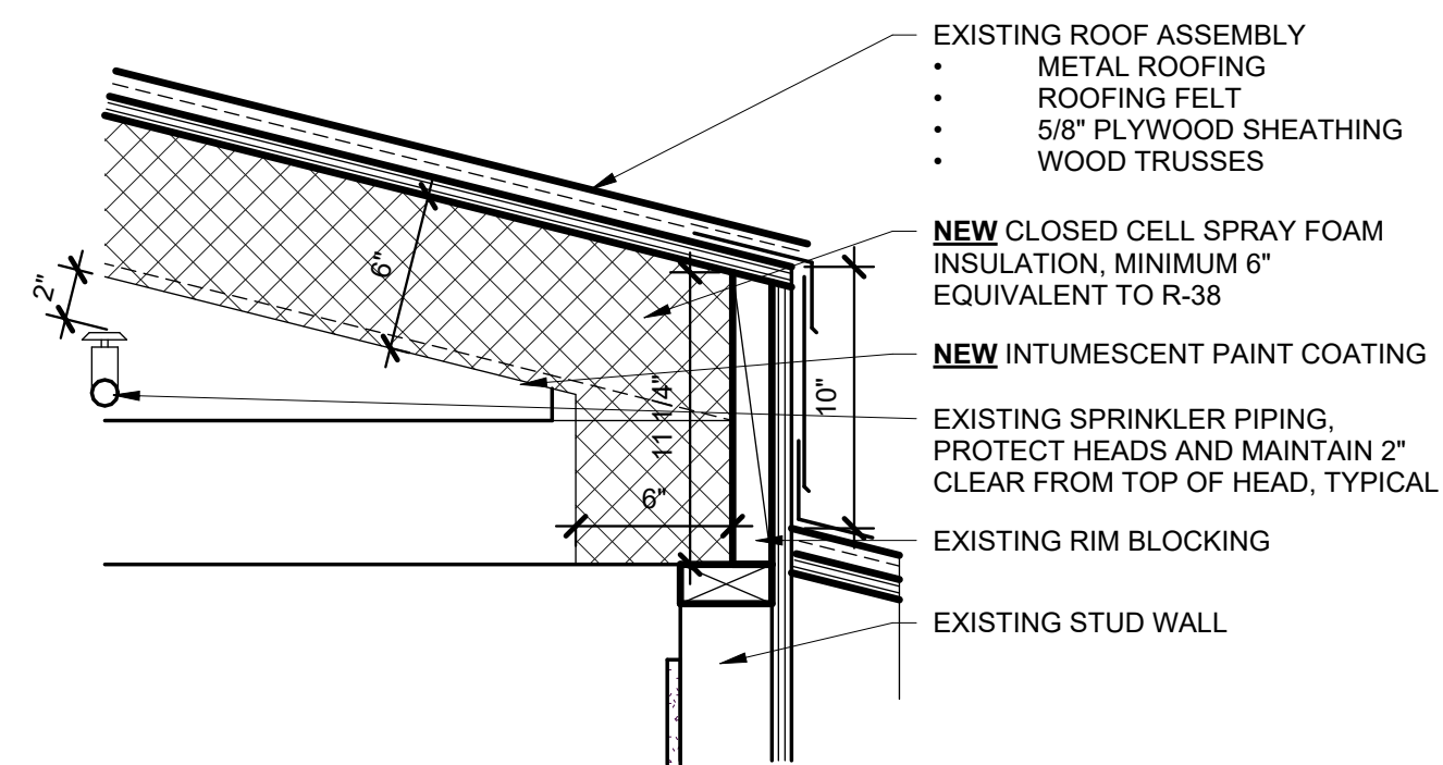
5 SPRAY FOAM AT EAVE 1 1/2" = 1'-0"
