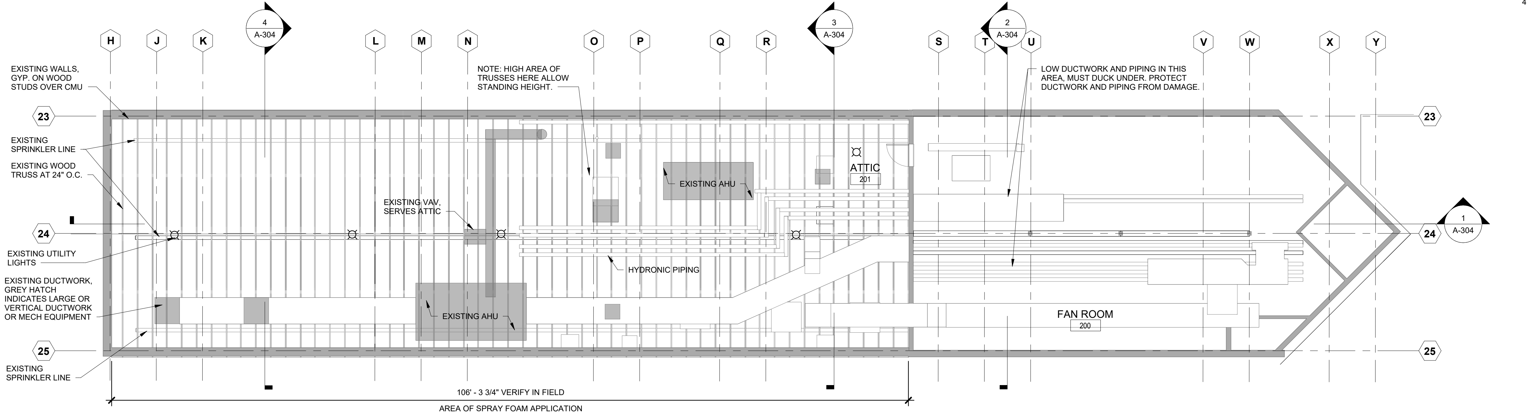
2 FAN ROOM REFLECTED CEILING PLAN 1/8" = 1'-0"
