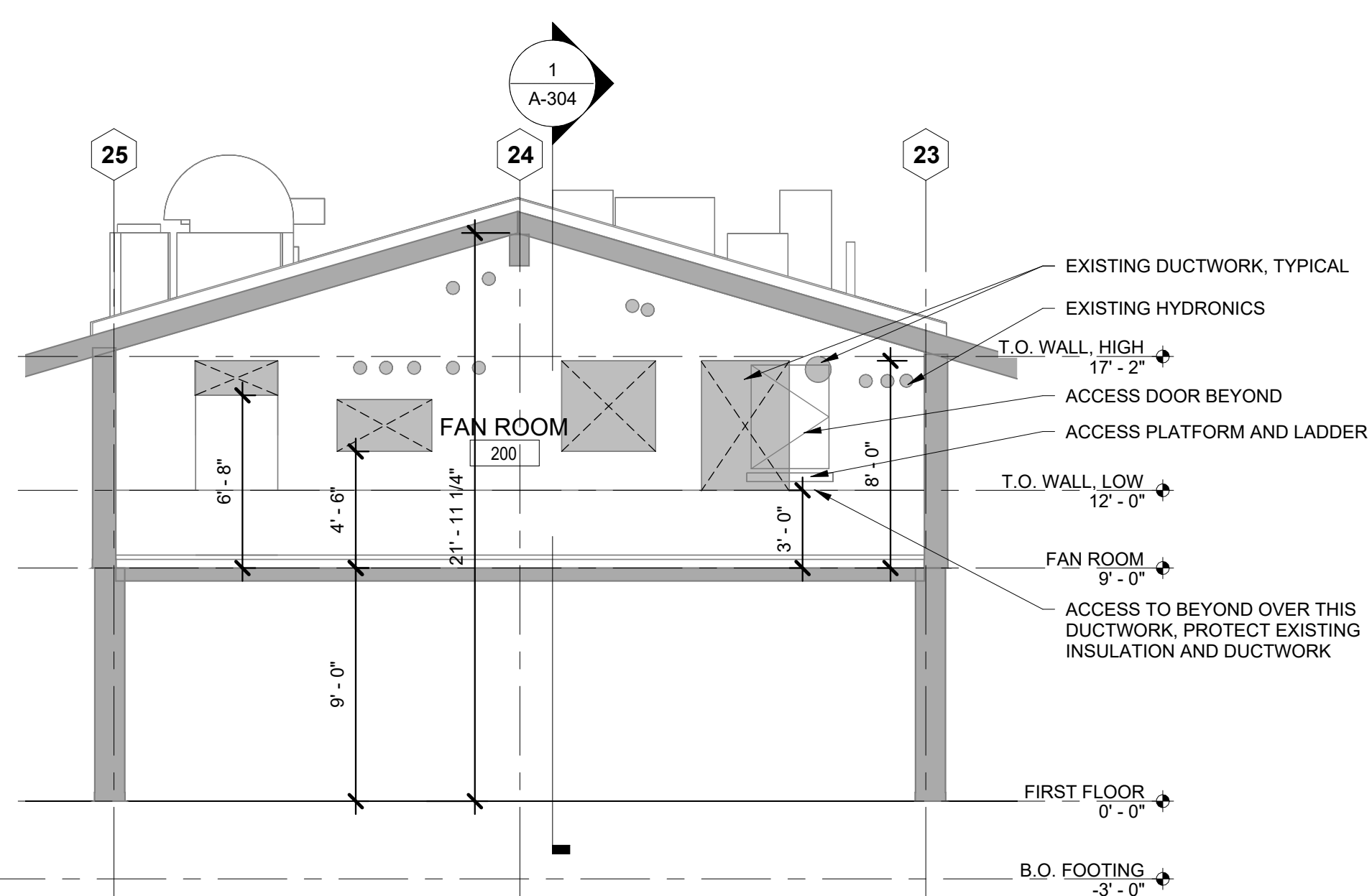
2 CROSS SECTION AT FAN ROOM 3/16" = 1'-0"
