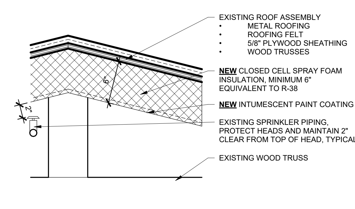
7 SPRAY FOAM AT EAVE 1 1/2" = 1'-0"
