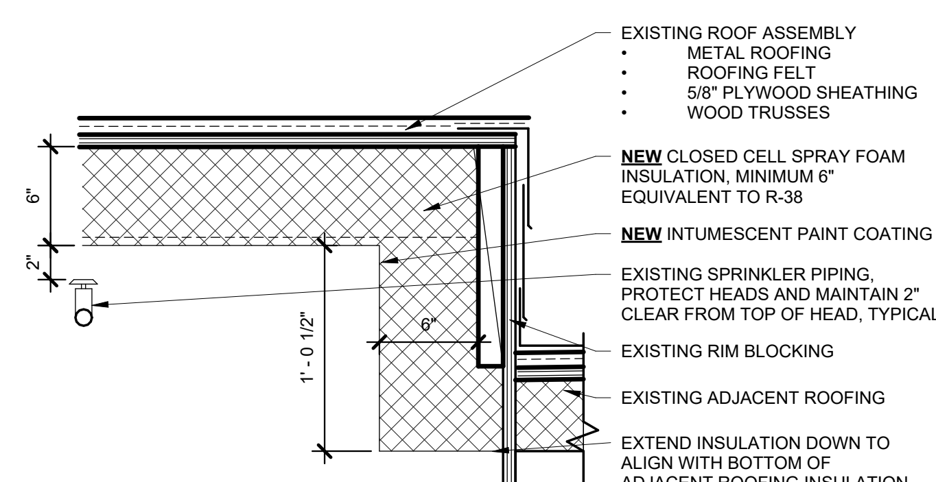
6 SPRAY FOAM AT RAKE 1 1/2" = 1'-0"
