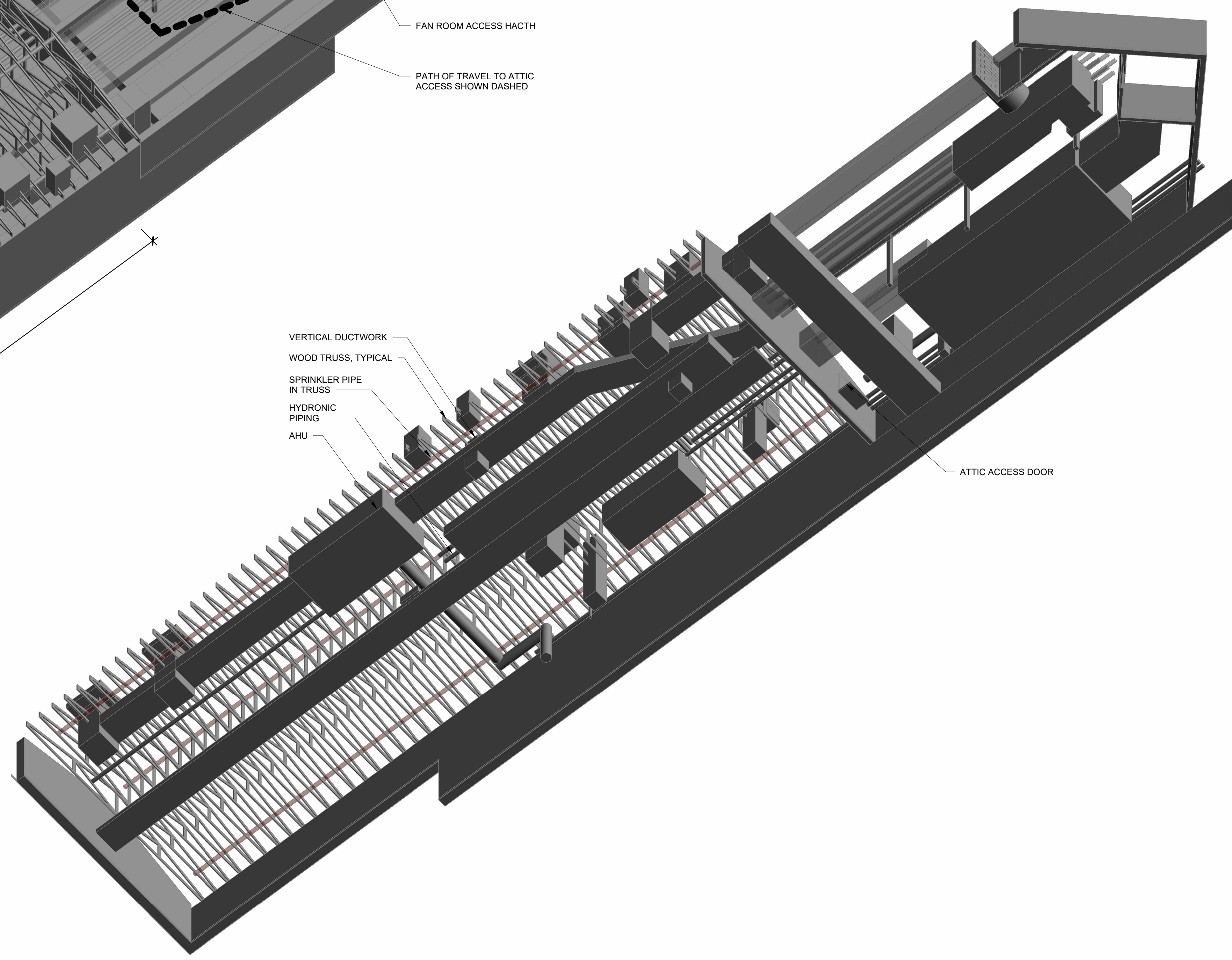
2 3D ISOMETRIC FAN ROOM FROM BELOW
