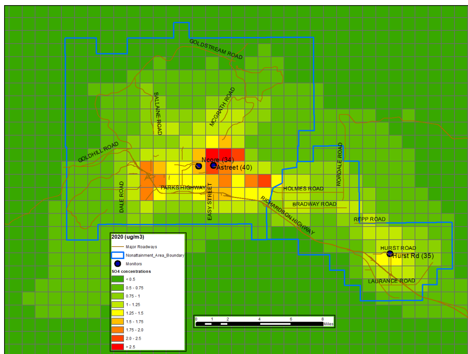
Figure 3.2.9 Sulfate ( \text{SO}_4 ) concentration plot in \mu\text{g}/\text{m}^3 at the surface for the Fairbanks NAA for the base year 2020
