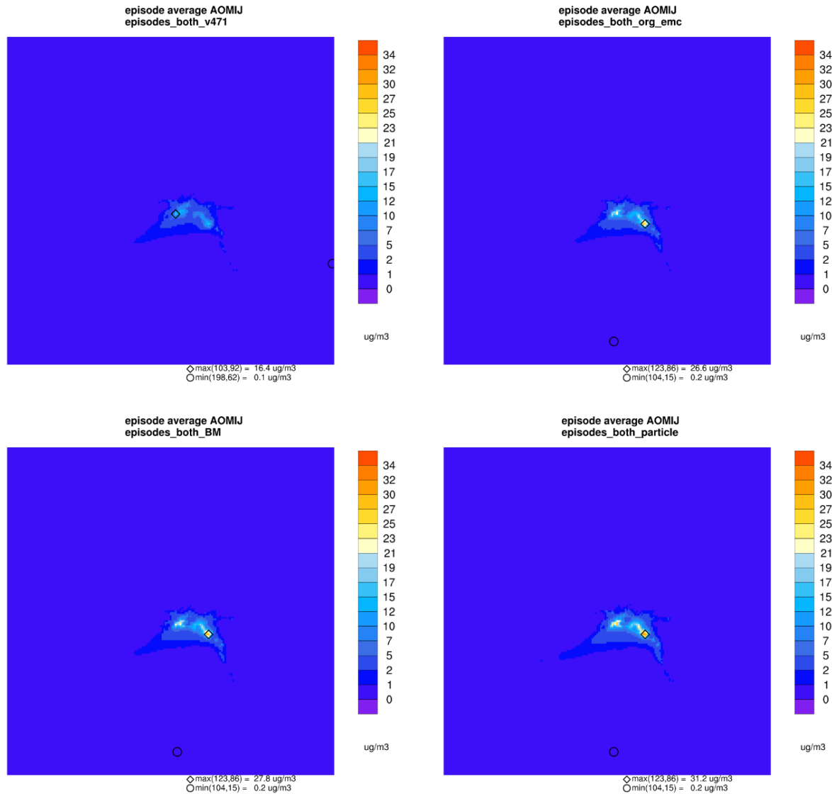
Figure 1.5.4 Organic Matter (AOMIJ) in \mu\text{g}/\text{m}^3 both episode average concentration in the domain area at 1.33 km grid cell for 2019 base year emissions inventory using CMAQ version 4.7.1 (top left), CMAQ version 5.3.2 ORG EMC (top right), BM (bottom left) and particle (bottom right)
