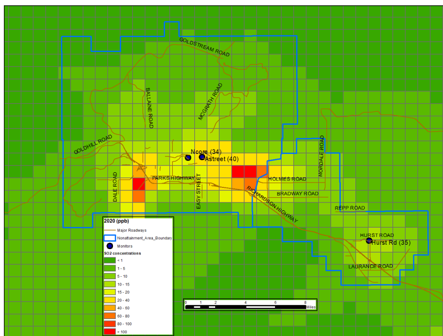
Figure 3.2.10 Sulfur dioxide (SO 2 ) concentration plot in ppb at the surface for the Fairbanks NAA for the base year 2020
