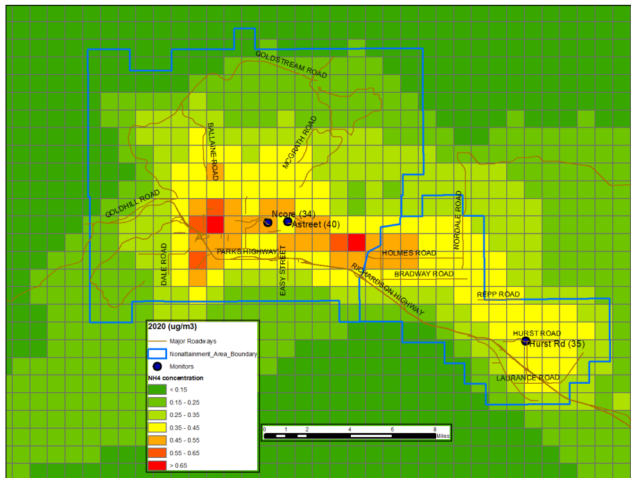
Figure 3.2.8 Ammonia ( \text{NH}_4 ) concentration plot in \mu\text{g}/\text{m}^3 at the surface for the Fairbanks NAA for the base year 2020
