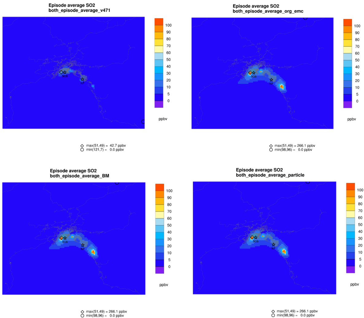
Figure 1.5.9 SO 2 in ppbv both episode average concentration in the domain area at 1.33 km grid cell for 2019 base year emissions inventory using CMAQ version 4.7.1 (top left), CMAQ version 5.3.2 ORG EMC (top right), BM (bottom left) and particle (bottom right)
