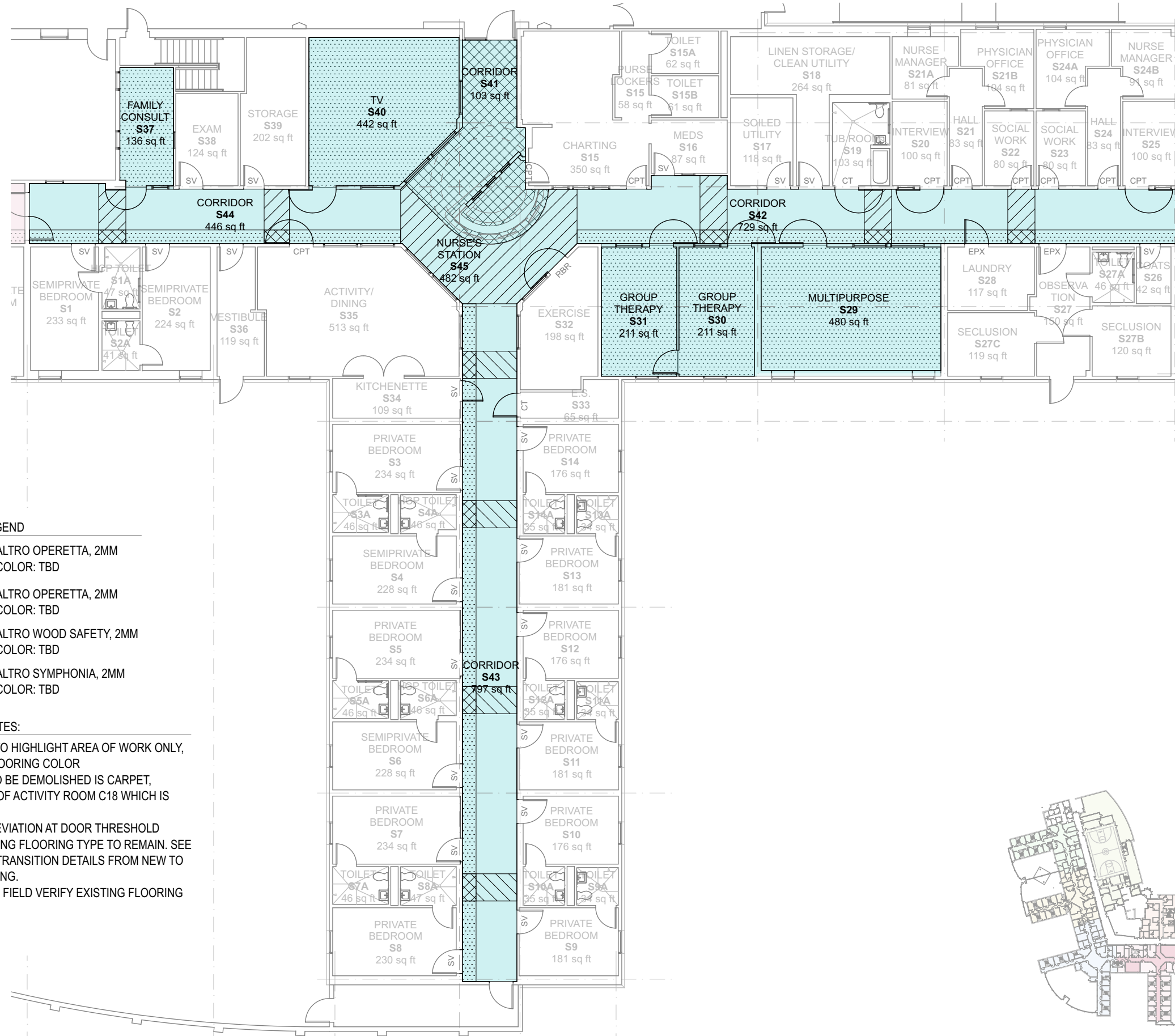
FLOOR FINISH PLAN - SUSITNA
