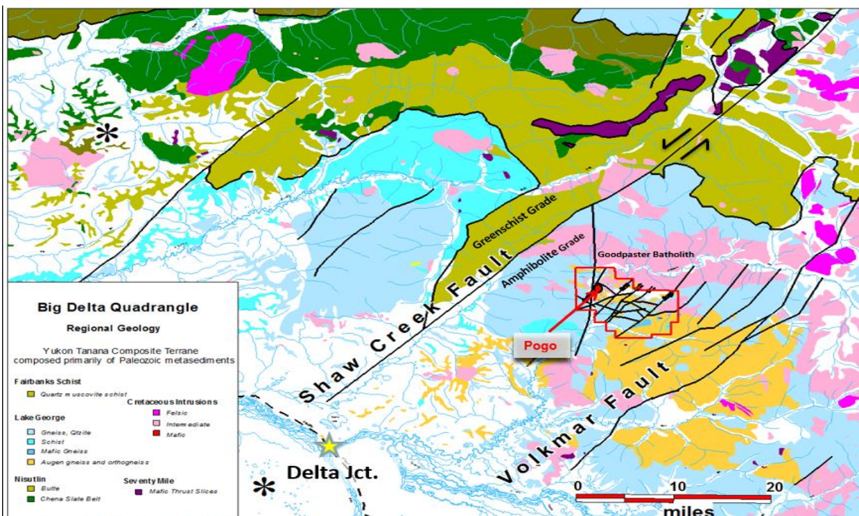
Figure 6.1.1 General Geology of the Pogo Project
