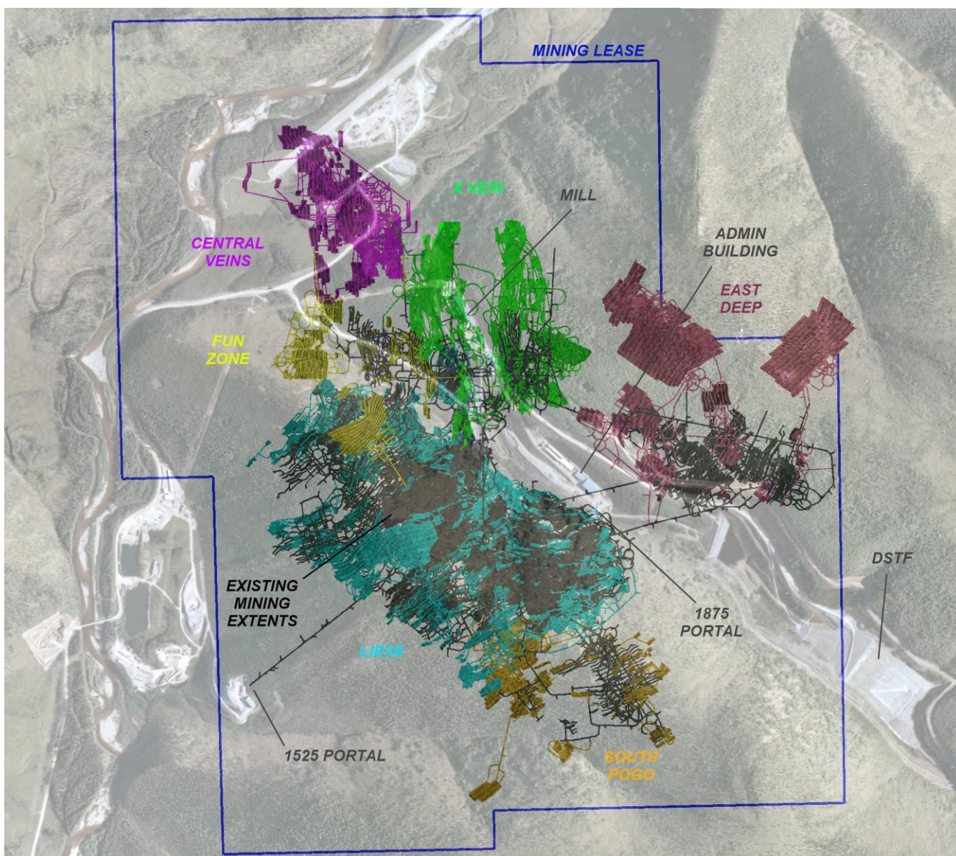
Figure 5.2.1: Plan View of Orebodies and Underground Development
