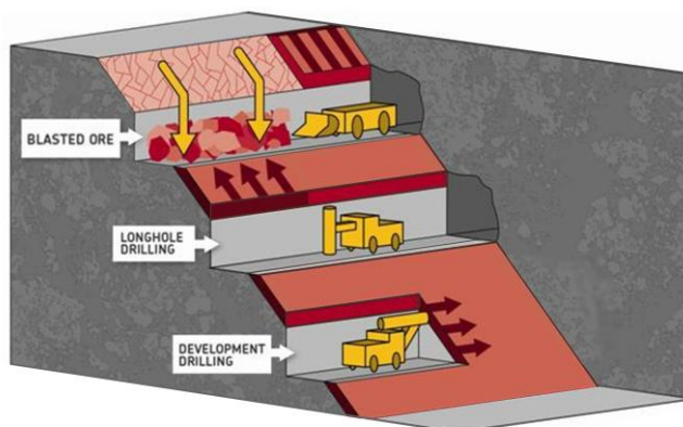
Figure 6.2.3: Longhole Open Stoping Cross-Section
