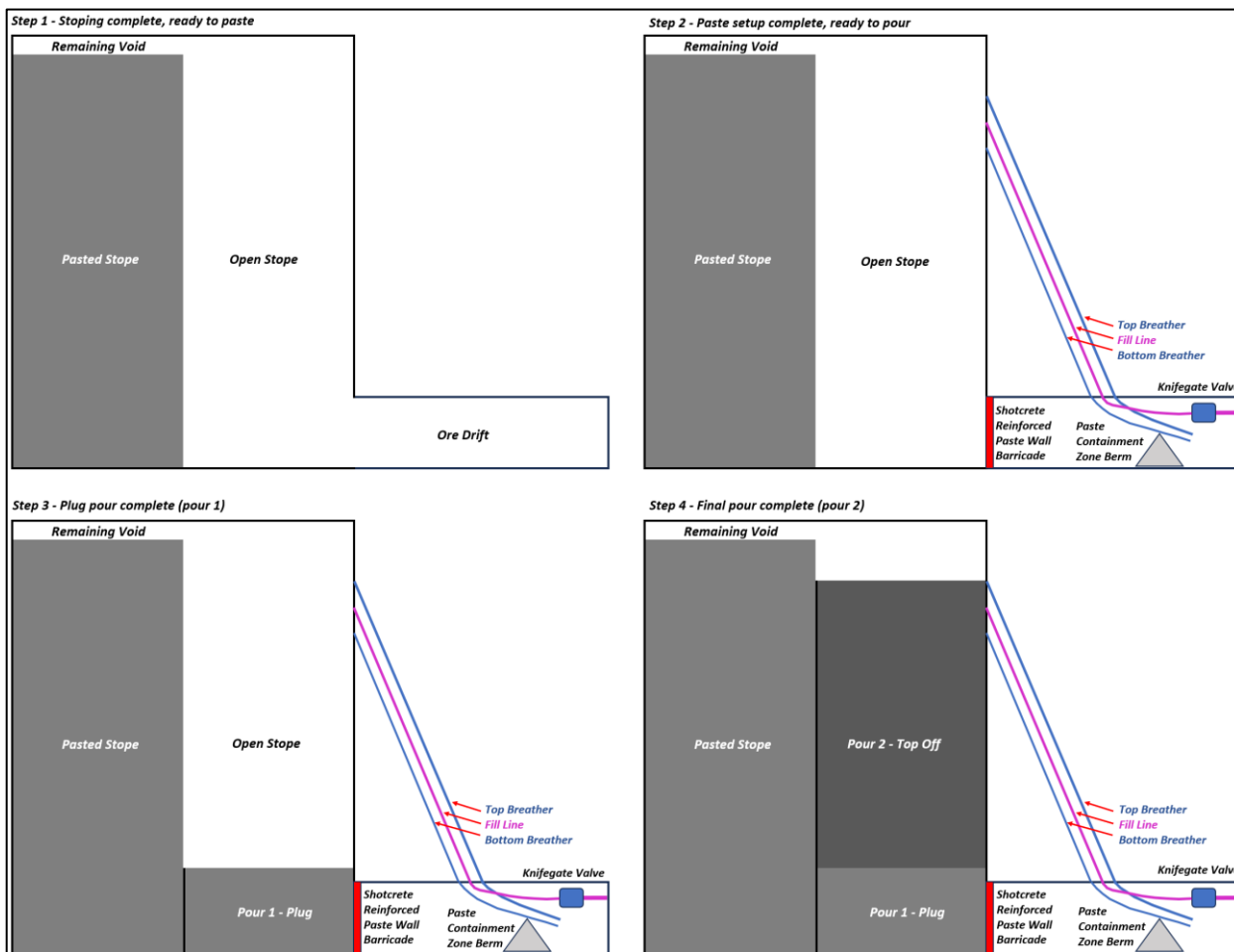
Figure 6.5: Backfill Cycle
