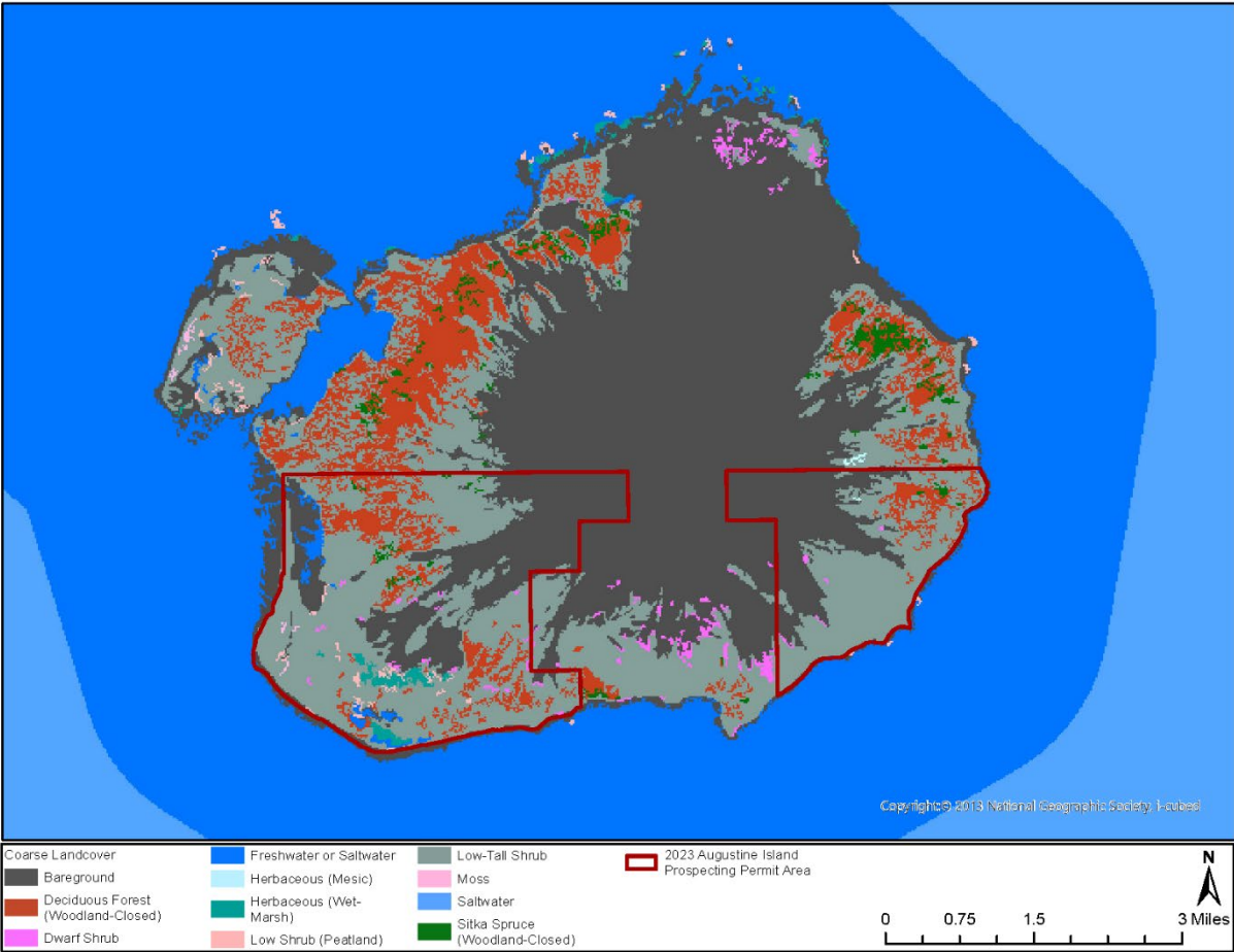
Figure 2. Landcover on Augustine Island.
