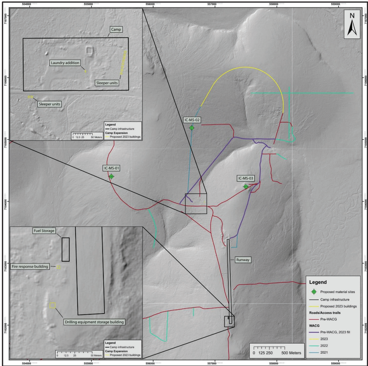
Figure 1. Location Map of Proposed Storage Buildings, Sleeper Cabins, and Material Sites
