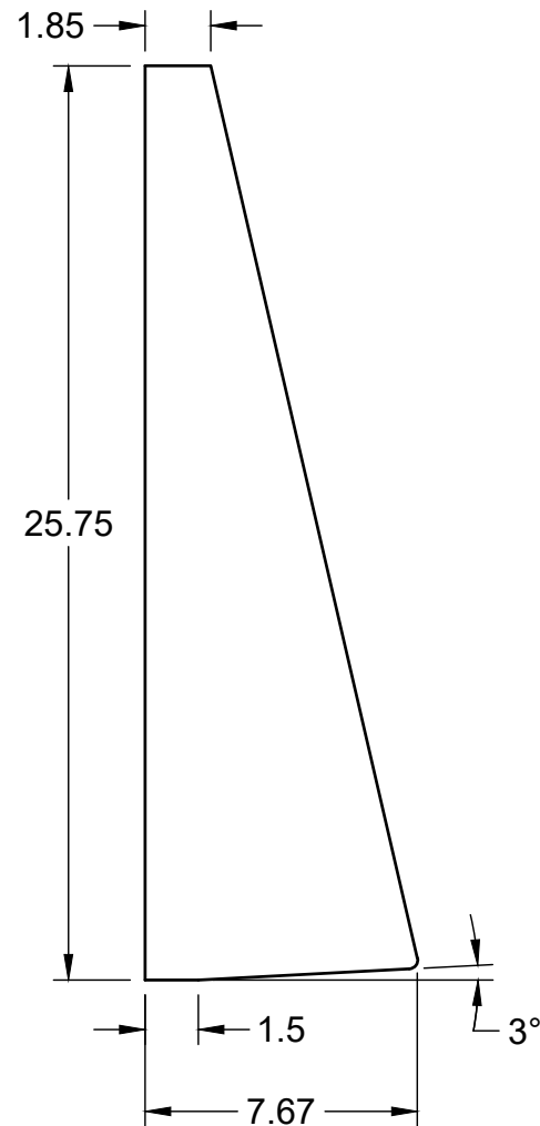
ARR 352 SINGLE SEAT FRAME UPPER TRIM BOARD - RIGHT PN: ARR-352-0012
