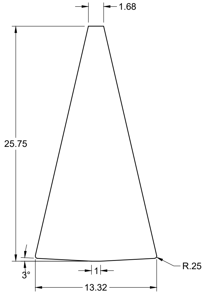
ARR 352 DOUBLE SEAT FRAME UPPER TRIM BOARD PN: ARR-352-0013
