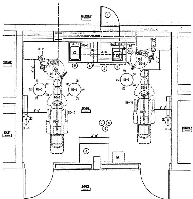
3 PARTIAL RENOVATION FLOOR PLAN - OPTION 3 SCALE: 1/2" = 1'-0" GRAPHIC SCALE 1/2" = 1'-0"
