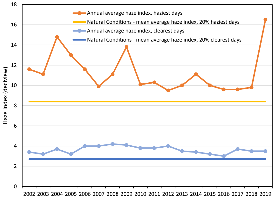
Figure 8.1. Haze index for conditions at Trapper Creek IMPROVE site, 2002 to 2019.
