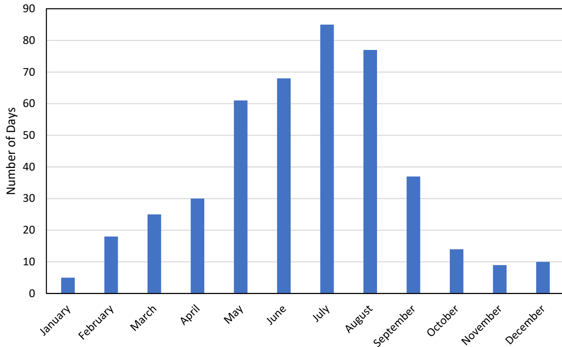
Figure 8.2. Distribution of haziest days 2001 to 2019 at the Trapper Creek IMPROVE station.
