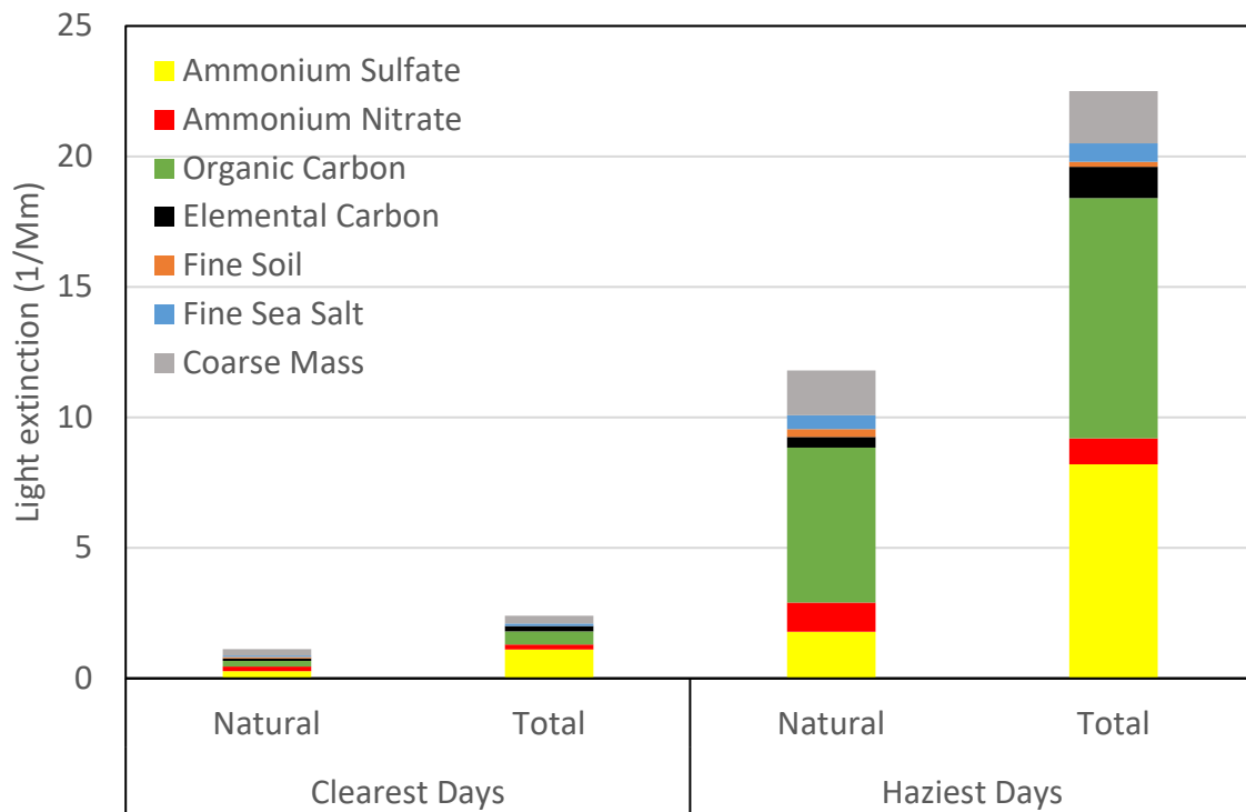
Figure 8.2. Distribution of haziest days 2001 to 2019 at the Trapper Creek IMPROVE station.
