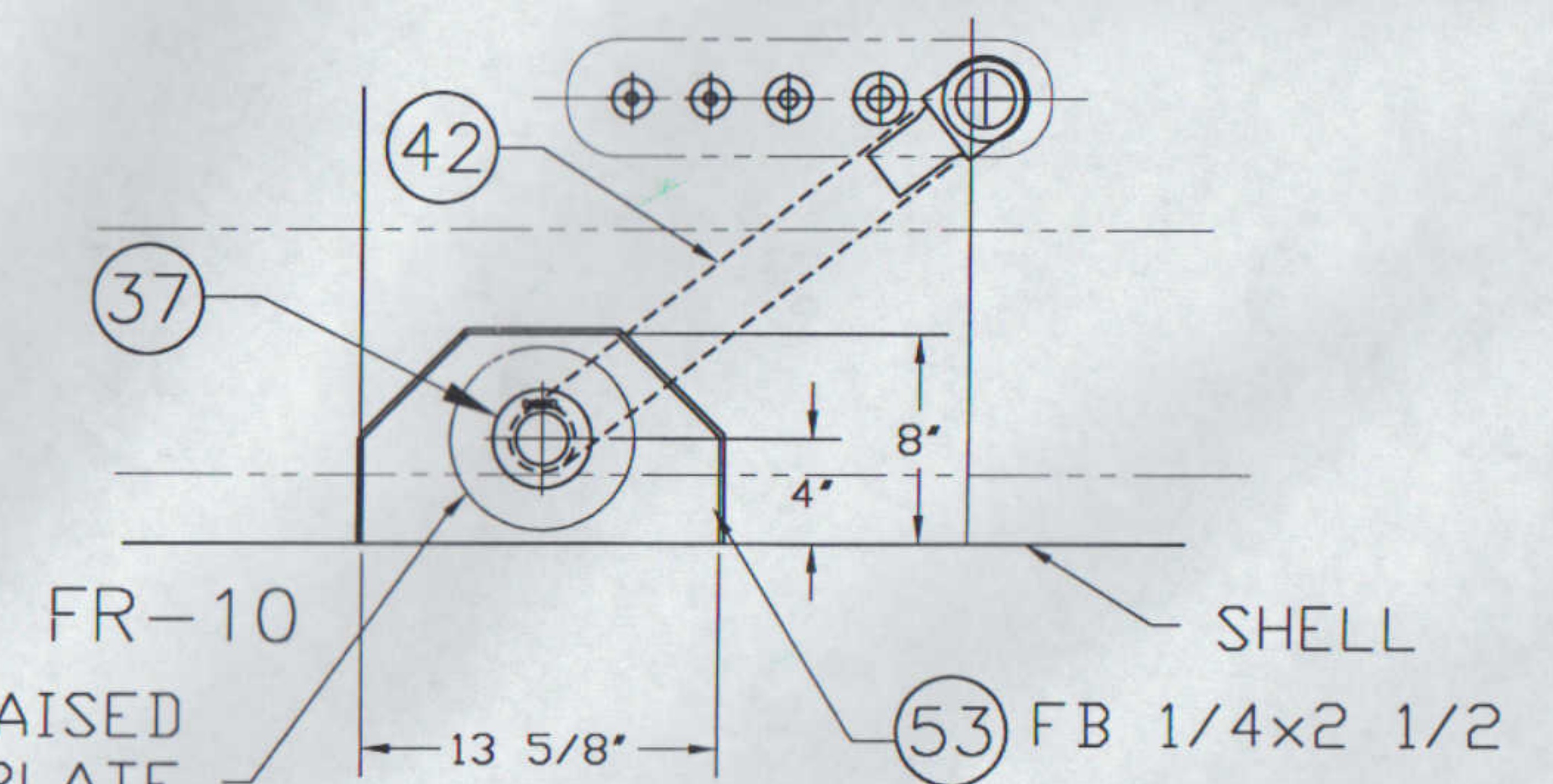
DETAIL - 1 SPILL COAMING SCALE: 1 1/2"=1'-0"
