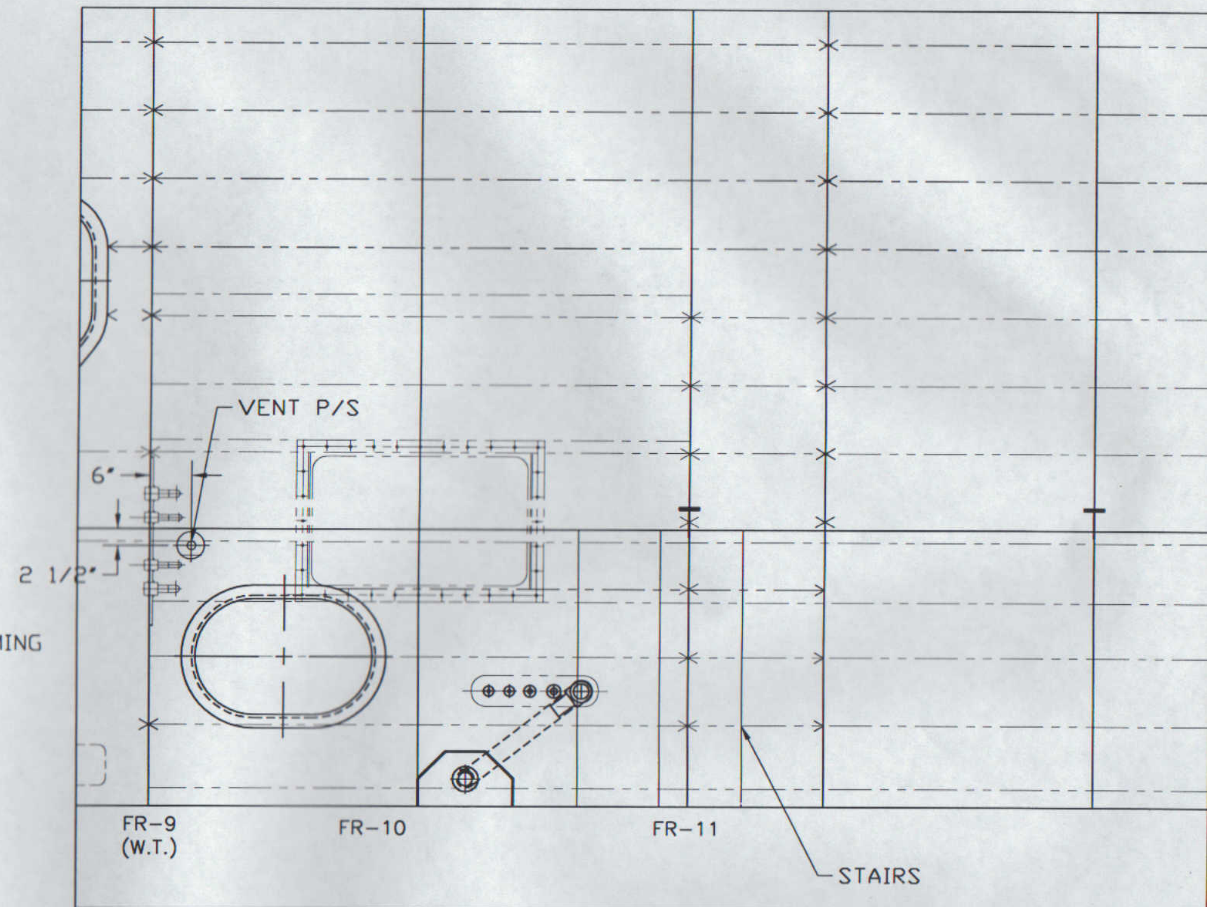
STBD PLAN VIEW
