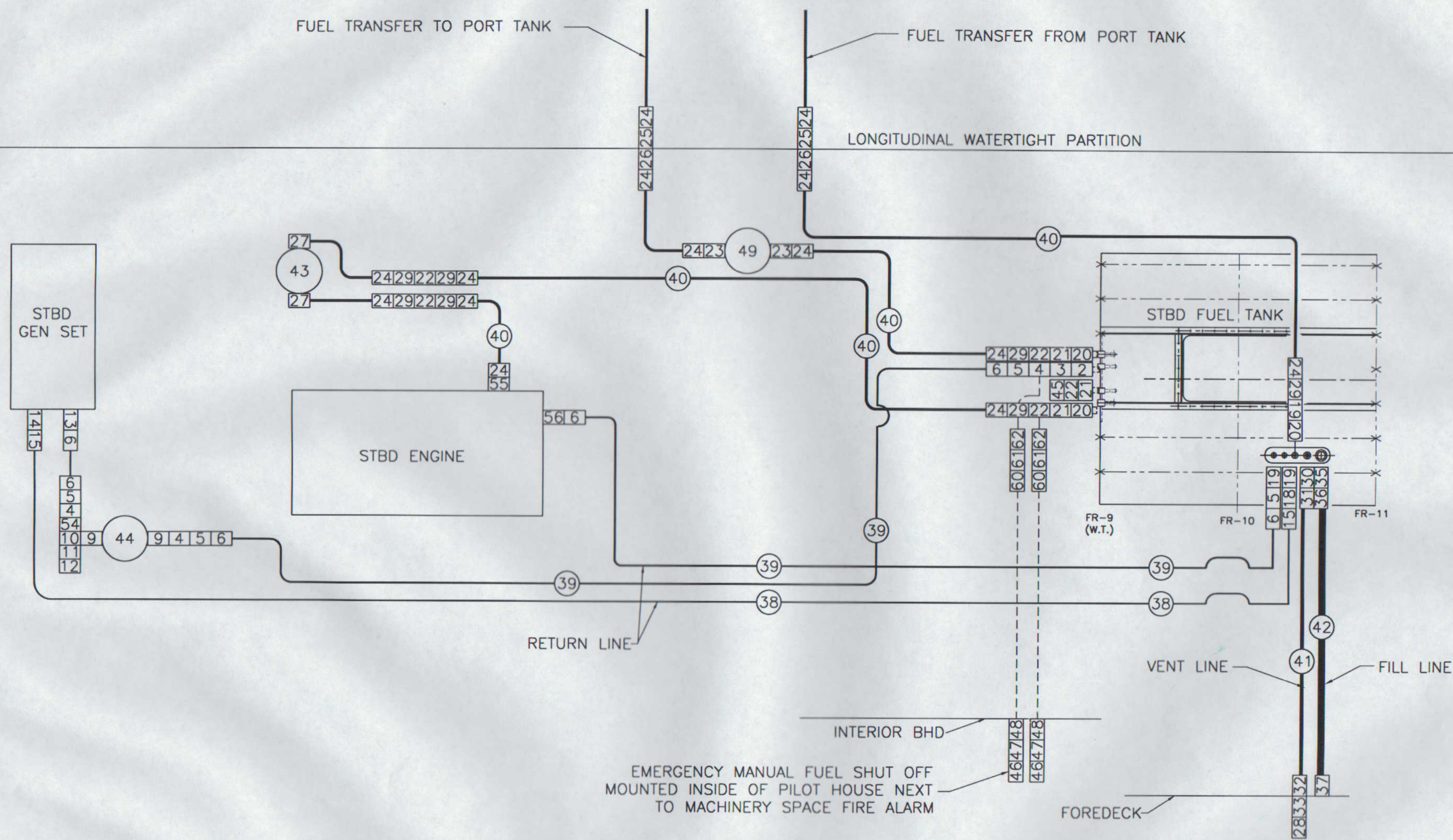
FUEL SYSTEM - STBD SIDE PORT SIDE SIMILAR
