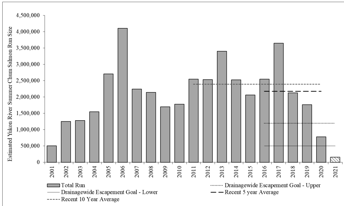
Figure 4.—Estimated Yukon River summer chum salmon run size. Run size from 2021 incorporates the escapement estimates into the Andreafsky River and a preliminary estimate of harvest based on years with fishing closures.
