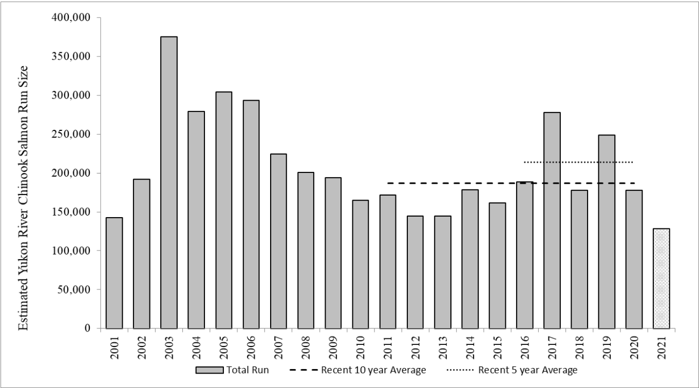
Figure 3.—Estimated Yukon River Chinook salmon run size. Run size from 2021 incorporates the escapement estimates into the Andreafsky River and a preliminary estimate of harvest based on years with fishing closures.
