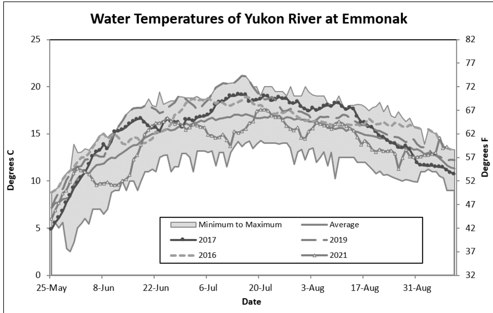
Figure 2.—Average daily water temperatures collected (from hand-held thermometers 1984–present and loggers 2004–2020) in the Yukon River near Emmonak, comparing 2021 and select years to historical minimum, maximum, and average temperatures. Measurements from 2021 were taken with a handheld thermometer and are preliminary.
