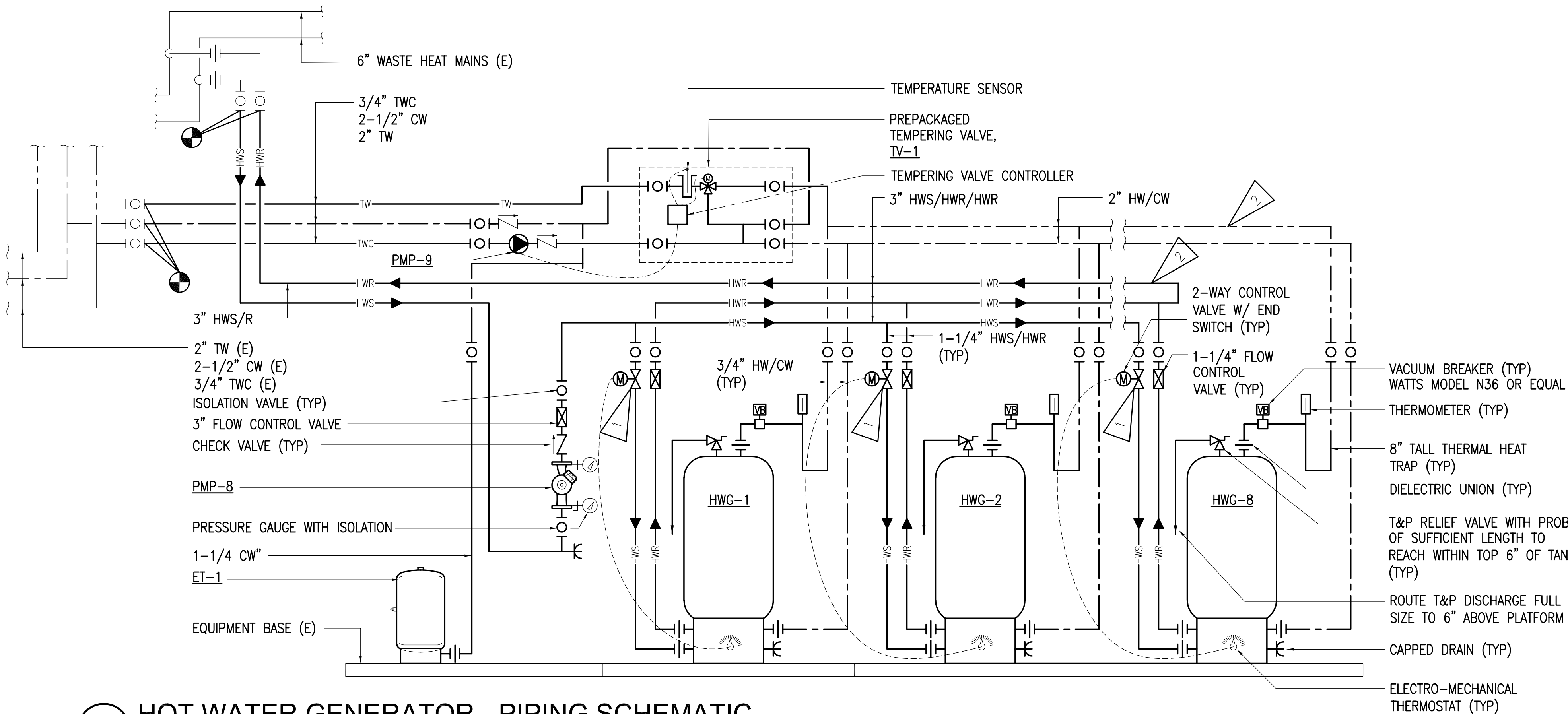
3 HOT WATER GENERATOR - PIPING SCHEMATIC NO SCALE
