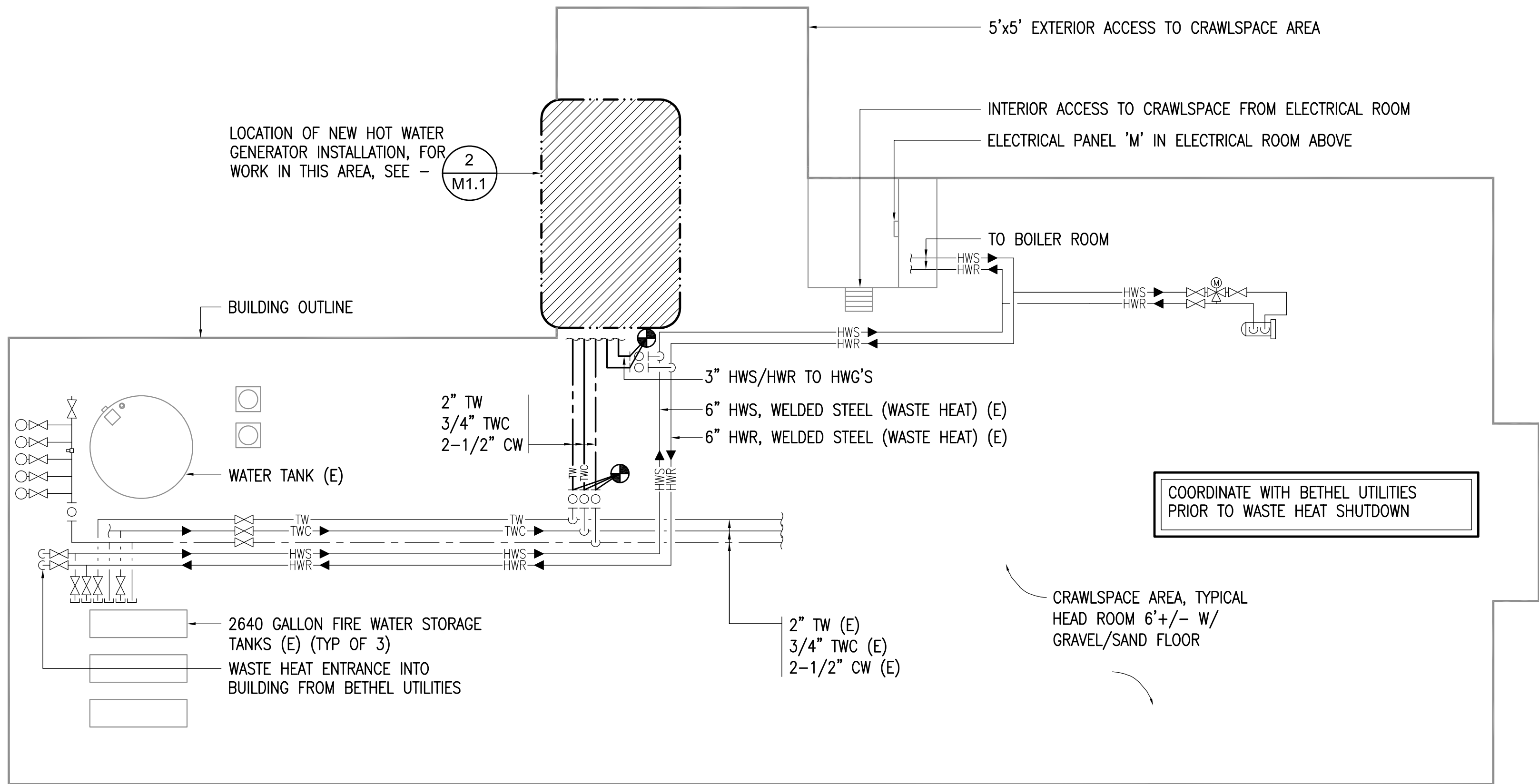
1 UNDERFLOOR BUILDING PLAN 1/16" = 1'-0"
