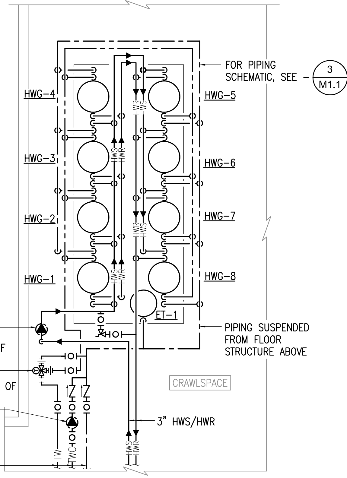
2 ENLARGED CRAWLSPACE PIPING PLAN 1/4" = 1'-0"
