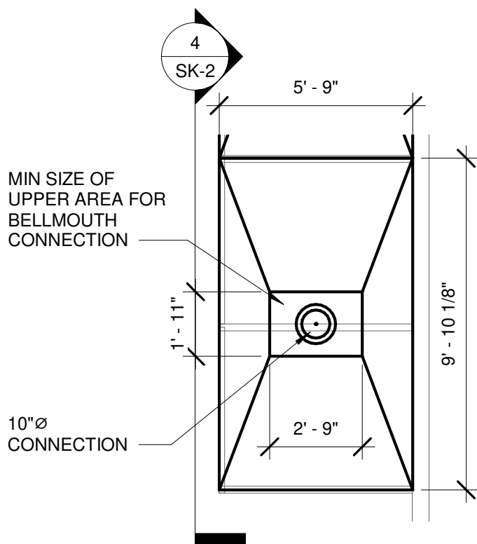
① DOUBLE HOOD TOP DETAIL 1/4" = 1'-0"
