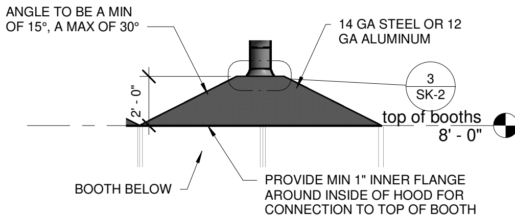
④ HOOD ELEVATION 1/4" = 1'-0"
