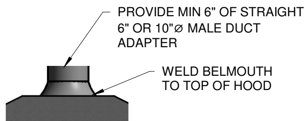
③ BELLMOUTH DETAIL 1/2" = 1'-0"
