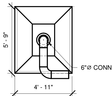
② SINGLE HOOD TOP 1/4" = 1'-0"
