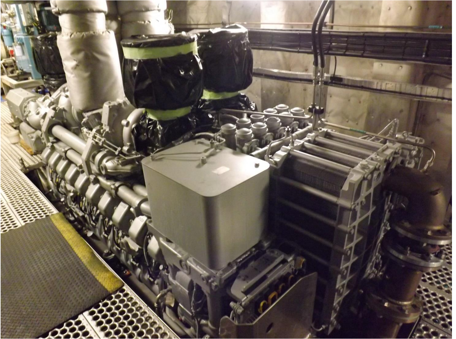
FVF Chenega Port Engine Room - MTU 20V 4000 M73L Engine ( U. S. EPA Tier 2 Certified )
