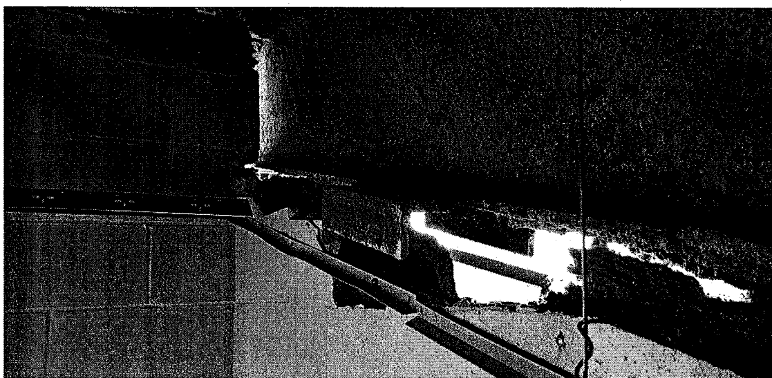
Figure 3 CMU Non-bearing Partition Wall Damage at Alpha 1 and Fox Mods Clerestory Area: Top of CMU Partition Wall
