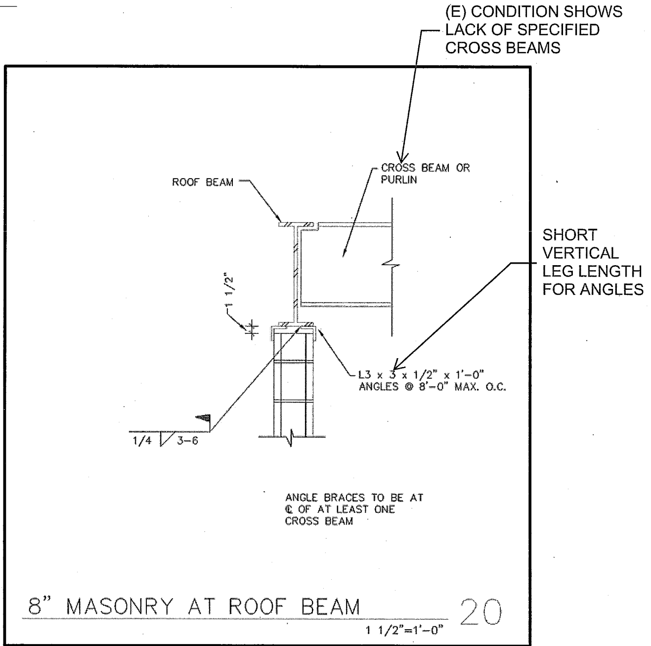
Figure 1 CMU Non-bearing Partition Wall Damage at Alpha 1 and Fox Mods Clerestory Area: Original Drawings
