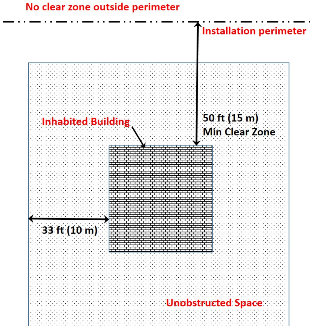
Figure 3-2 Installation Perimeter without Outer Clear Zone
