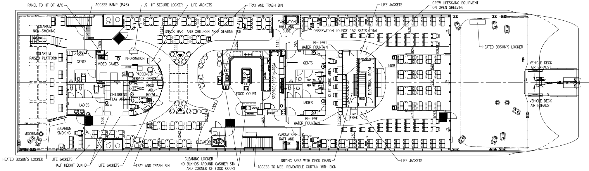
DECK 03 (PASSENGER DECK)
