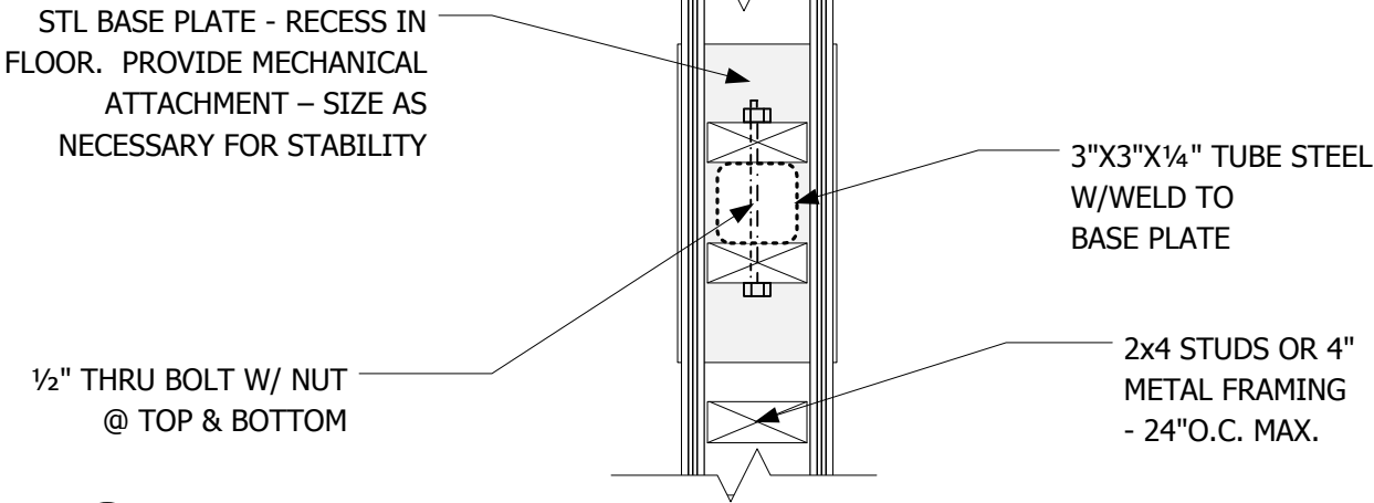
AA SECTION AA
