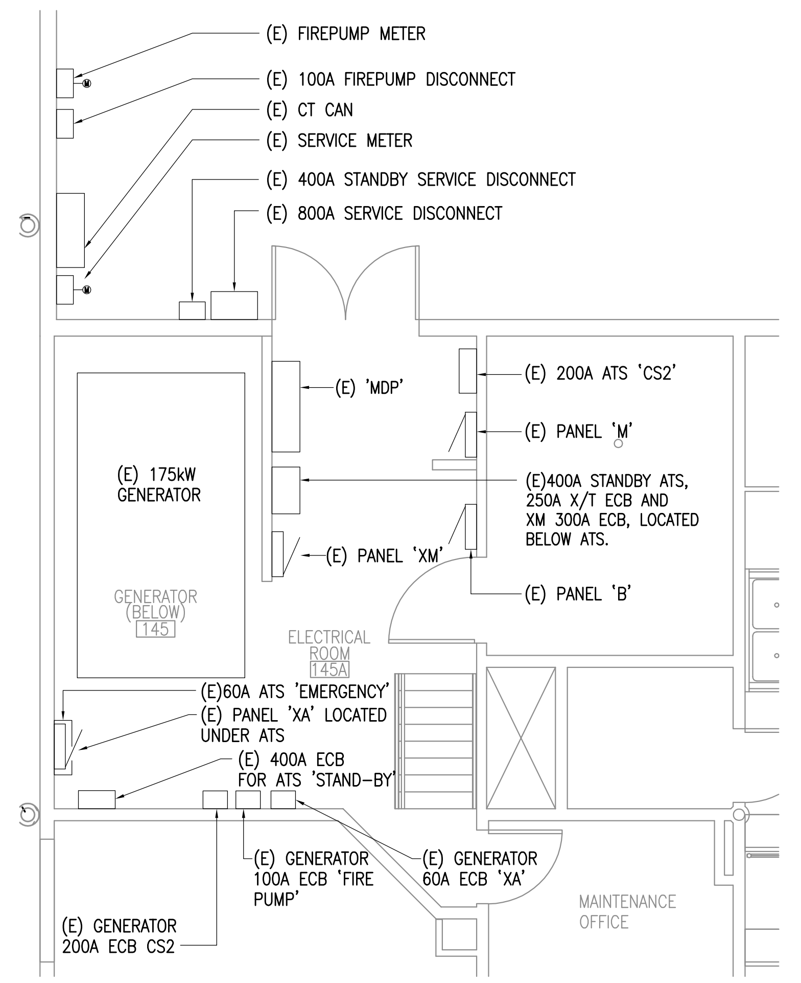
3 ENLARGED PARTIAL PLAN MAIN FLOOR - PANEL MAP 1/4" = 1'-0"
