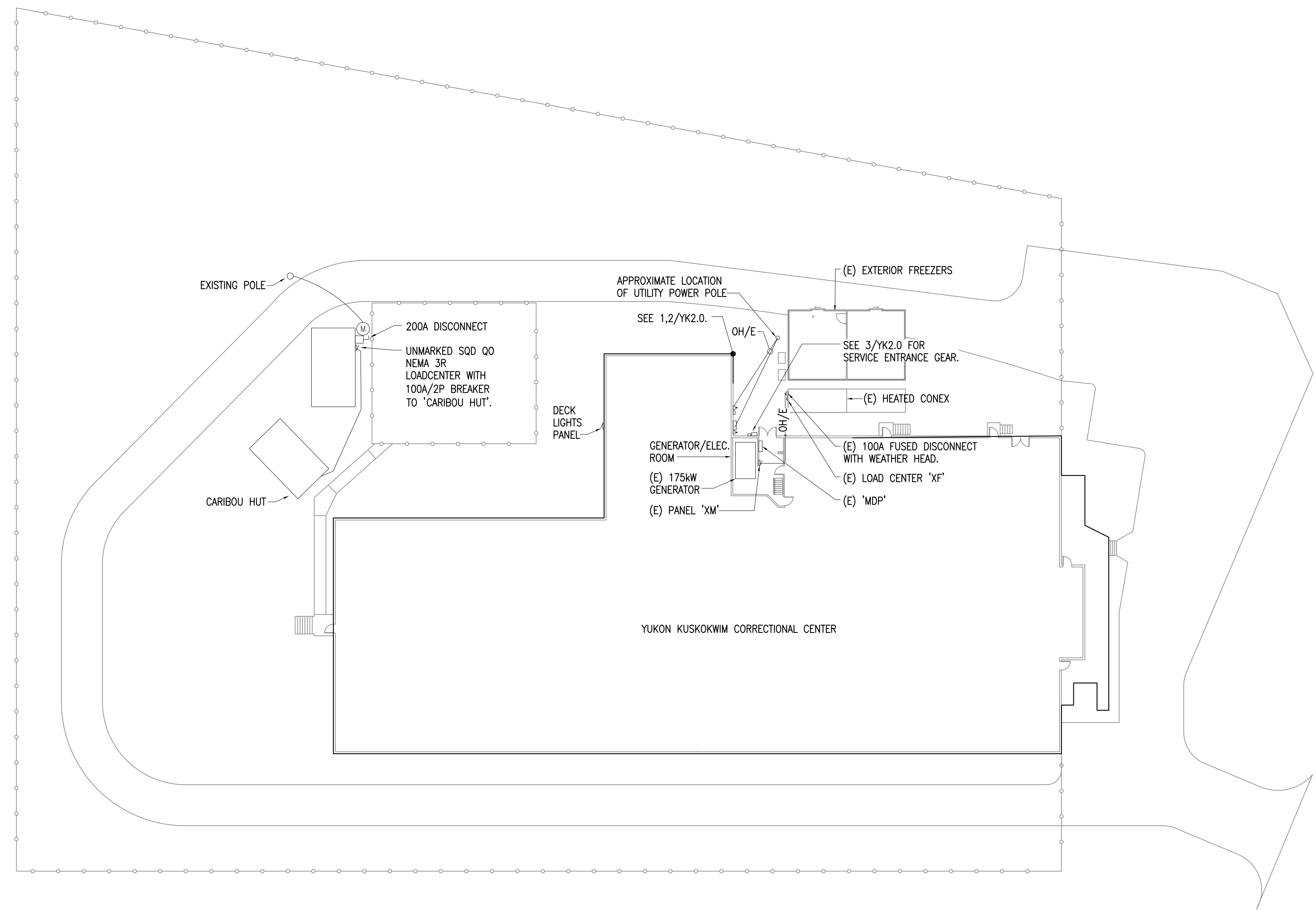
1 YKCC BUILDING MAP - SITE 1" = 20' - 0"
