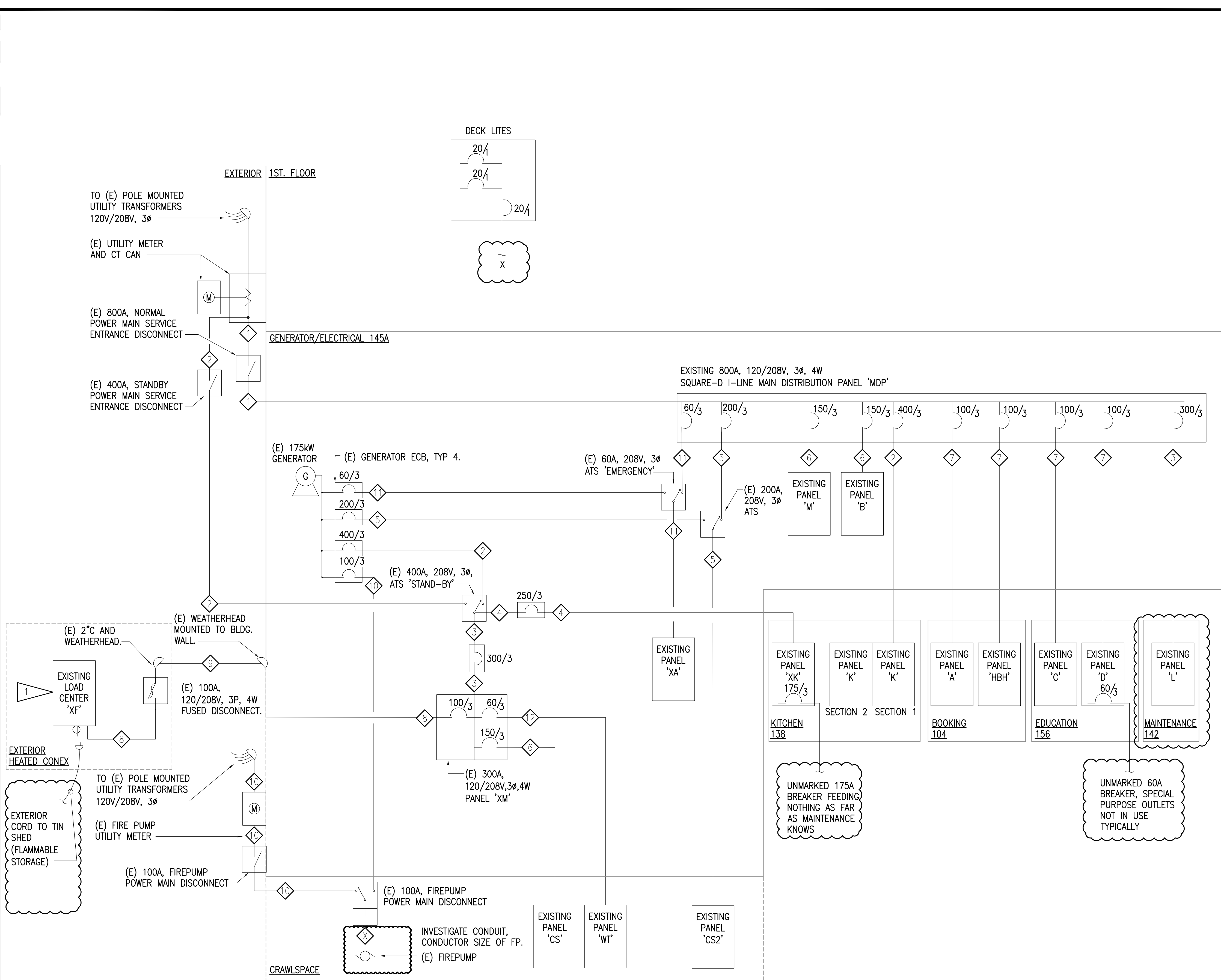
1 YKCC POWER ONE-LINE DIAGRAM
