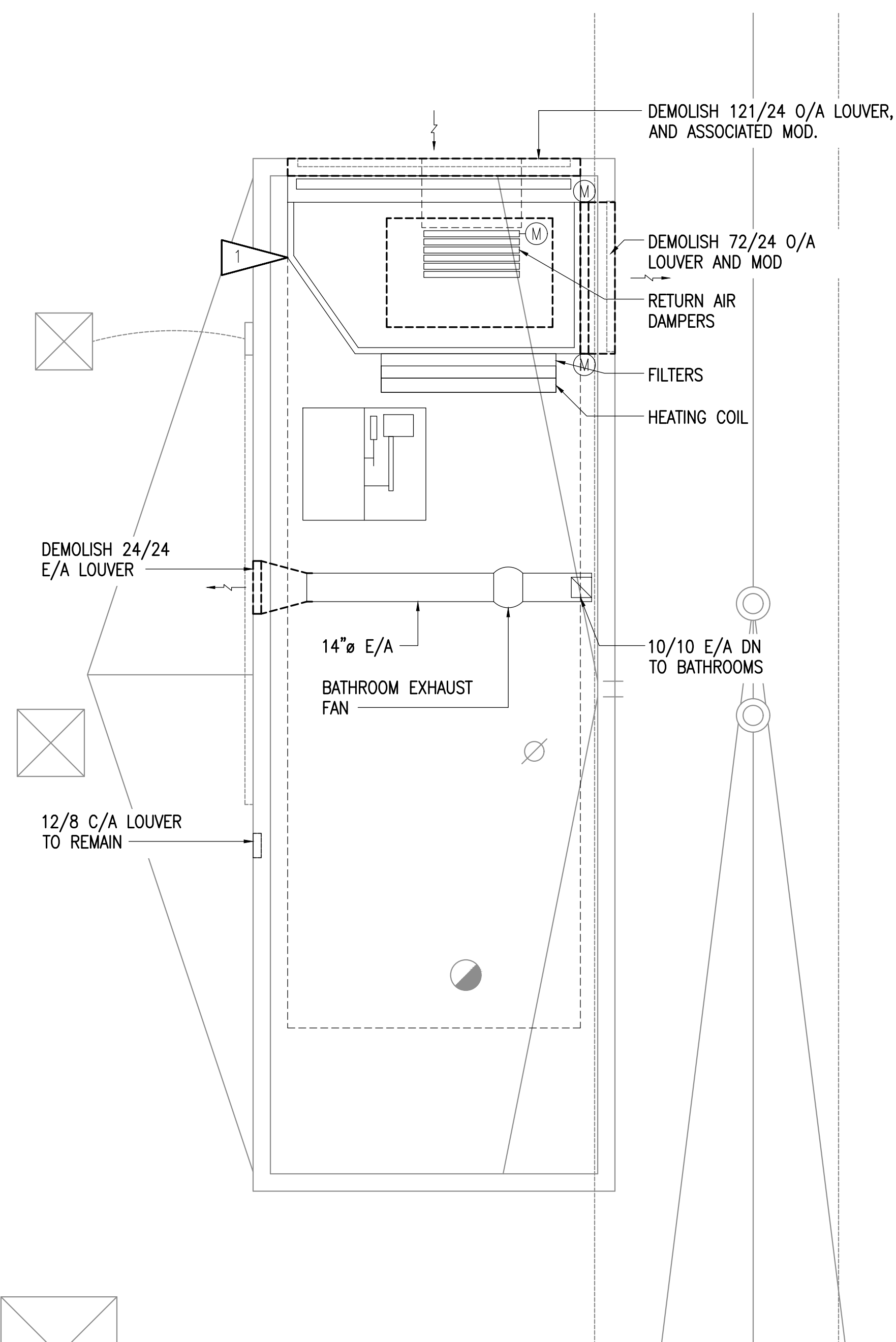
1 ENLARGED PENTHOUSE DEMOLITION PLAN - SOUTH 1/4"=1'-0"
