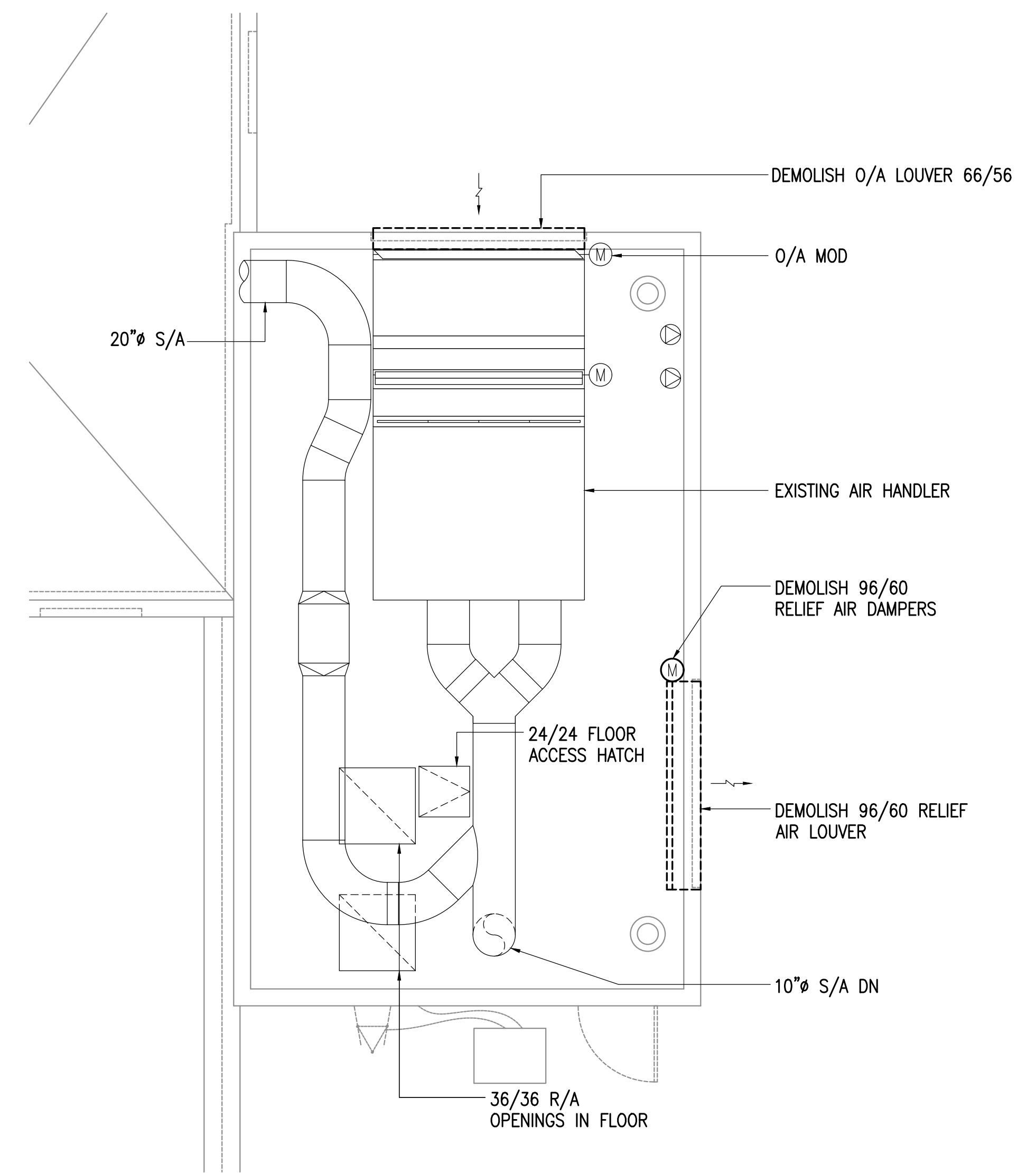
2 ENLARGED PENTHOUSE DEMOLITION PLAN - NORTH 1/4"=1'-0"
