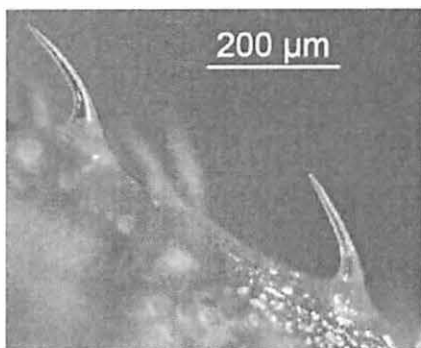
Cystolithic trichomes
