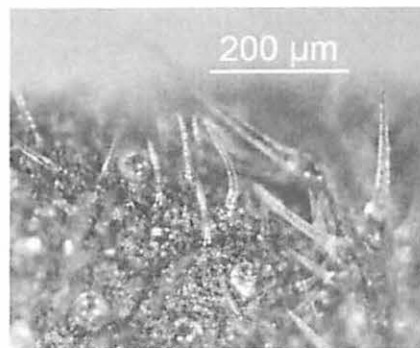
Non-cystolithic trichomes
